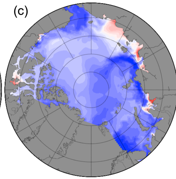
ORCA025
