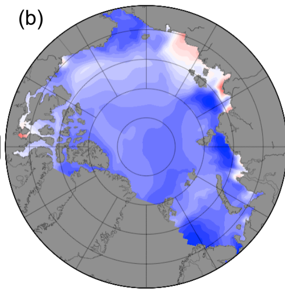
ORCA05
