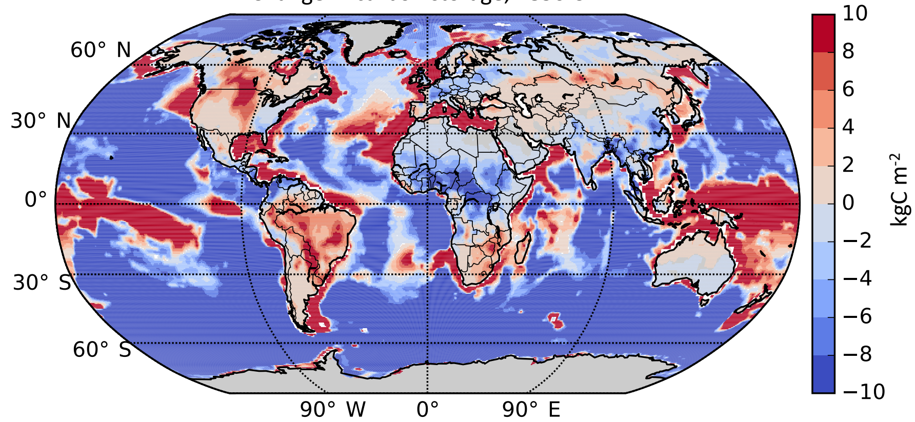
Change in carbon storage, 1850 CE
