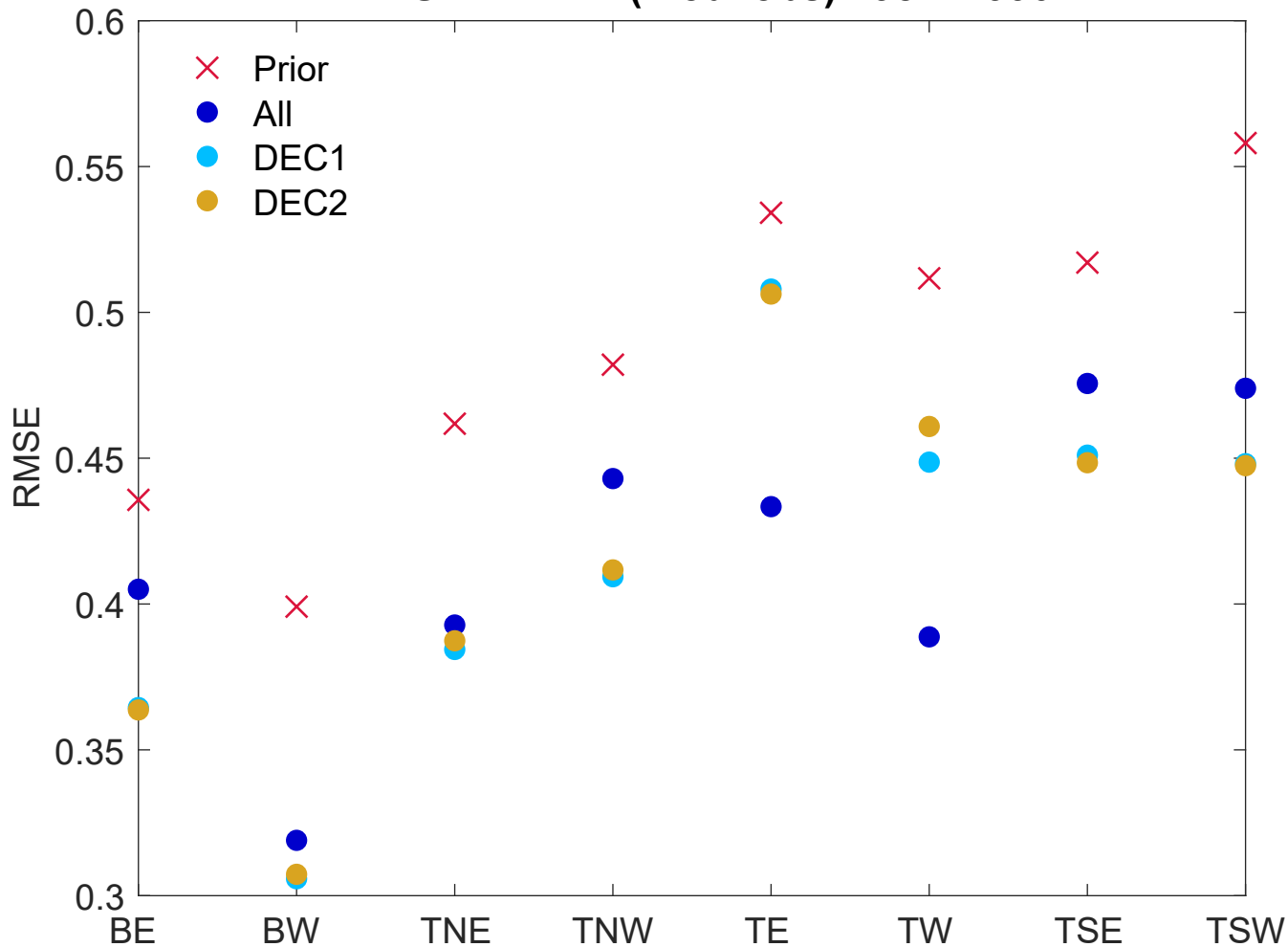
RMSE FAPAR (mod-obs) 1982-1990
