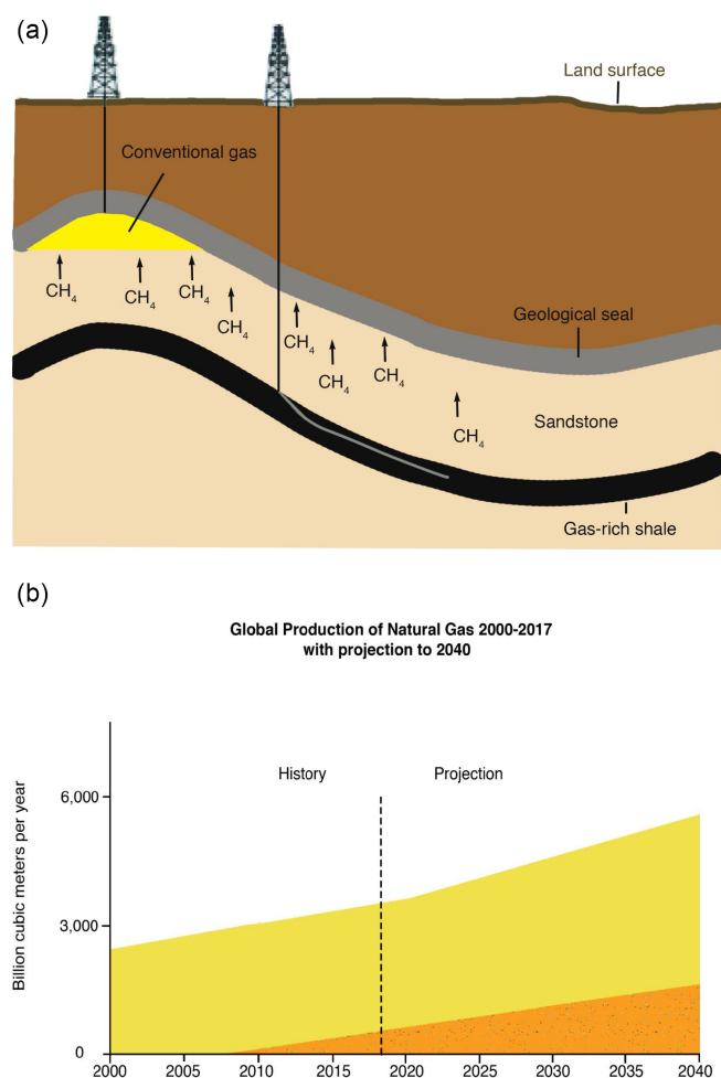
Figure 2. (a) Schematic comparing shale gas and conventional natural gas. For conventional natural gas, methane migrates from the shale through semipermeable formations over geological time, becoming trapped under a geological seal. Shale gas is methane that remained in the shale formation and is released through the combined technologies of high-precision directional drilling and high-volume hydraulic fracturing. (b) Global production of shale gas and other forms of natural gas from 2000 to 2017, with projections into the future from EIA (2016). Redrawn from EIA (2016) with data from IEA (2017).
