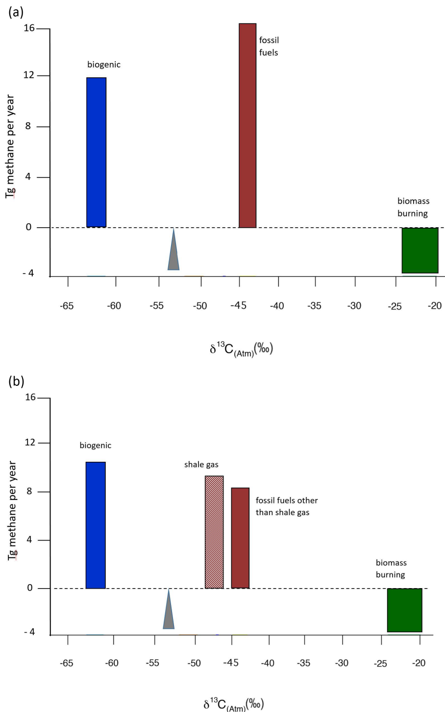
Figure 3. (a) On the x axis, \delta^{13}\text{C} values for methane from biogenic sources, fossil fuel, and biomass burning as presented in Worden et al. (2017) for values from Schwietzke et al. (2016); width of horizontal bars represents the 95 % confidence limits for these values. Triangle indicates the flux-weighted mean input of methane to the atmosphere. The y axis shows mean estimates from Worden et al. (2017) for the increase and decrease in methane emissions from particular sources since 2007 as calculated using the \delta^{13}\text{C} values of Schwietzke et al. (2016). (b) On the x axis, \delta^{13}\text{C} values as in Fig. 3a, except the value for fossil fuels does not include shale gas and a separate estimate for shale-gas value is included (see text). The y axis indicates estimates developed in this paper for the increase or decrease in methane emissions since 2008.
