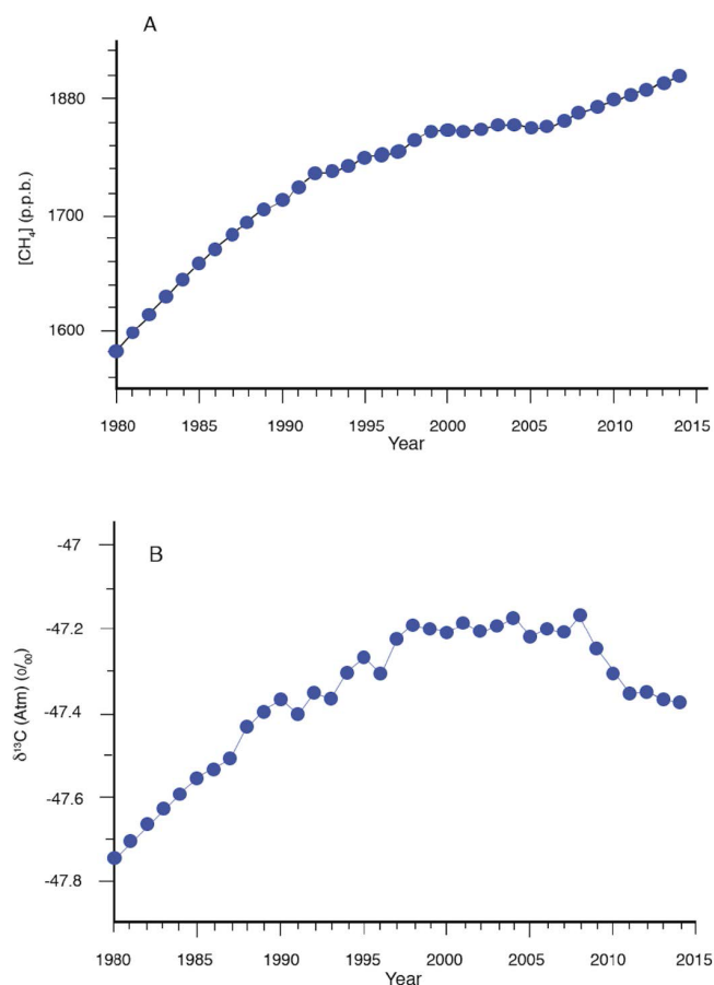
Figure 1. (a) Global increase in atmospheric methane between 1980 and 2015. (b) Change in \delta^{13}\text{C} value of atmospheric methane globally between 1980 and 2015. Both adapted from Schaefer et al. (2016).
