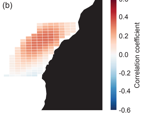
Corr.(NAO, F_{CO_2} ) ensemble mean
