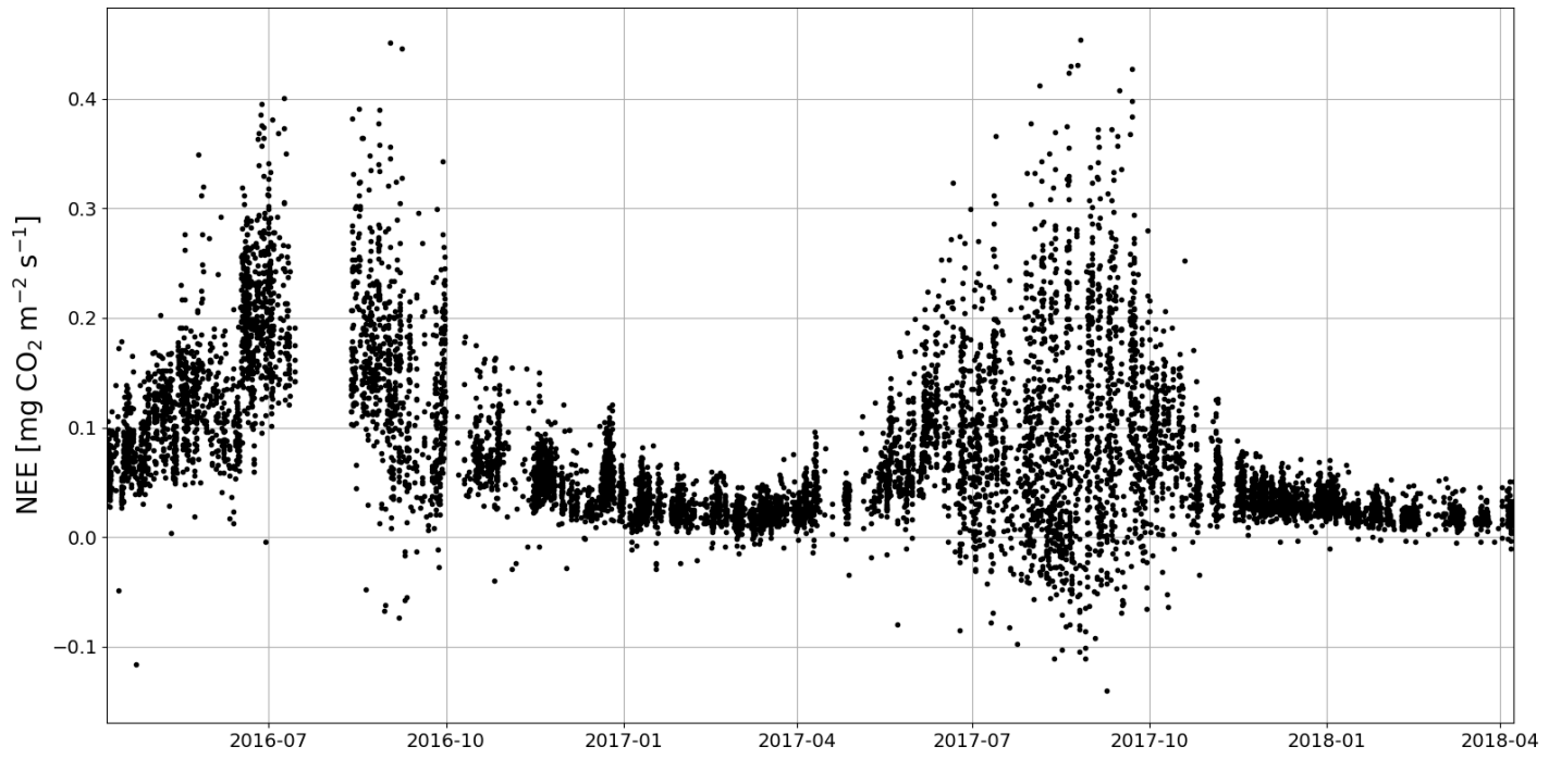
Figure S2. Time series of the accepted half-hourly measurements of NEE in April 2016 – April 2018.
