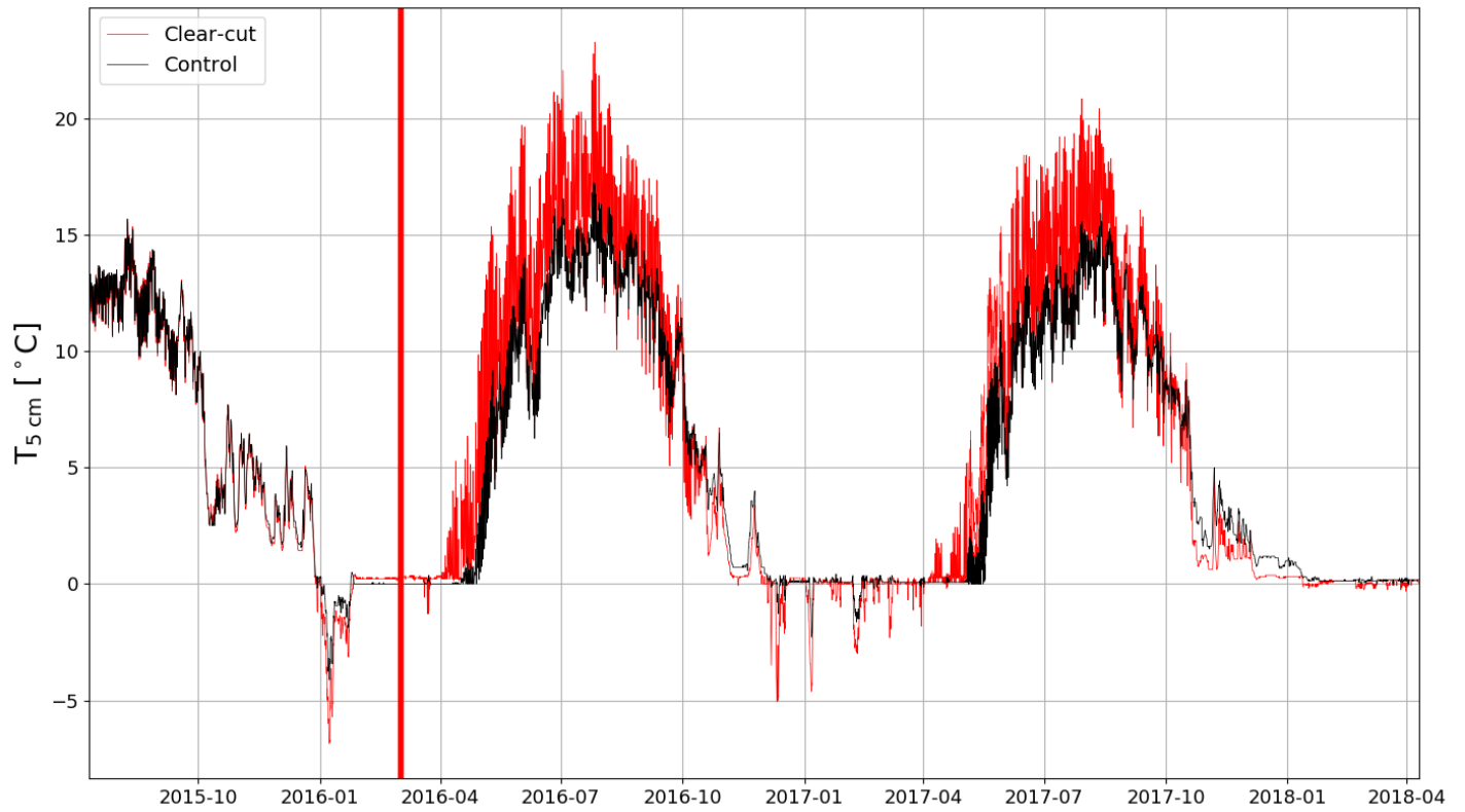
Figure S4. Hourly mean soil temperatures at 5 cm depth measured at the clear-cut (red) and the control (black) treatments. The clearcutting (red vertical line) was carried out in February–March 2016.
