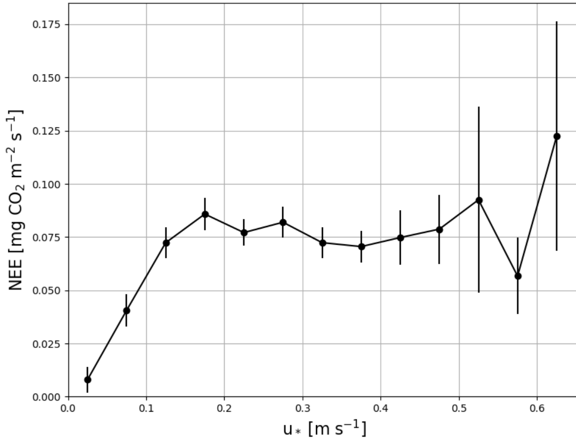
Figure S1. Average night-time (PPFD < 20 \mu\text{mol m}^{-2} \text{ s}^{-1} ) \text{CO}_2 flux ( \pm 95\% confidence interval) in the whole measurement period (4/2016 – 9/2017) as a function of friction velocity. The data were grouped into u_* bins of 0.05 \text{ m s}^{-1} . The u_* limit below which the data were rejected for further analysis was set to 0.125 \text{ m s}^{-1}
