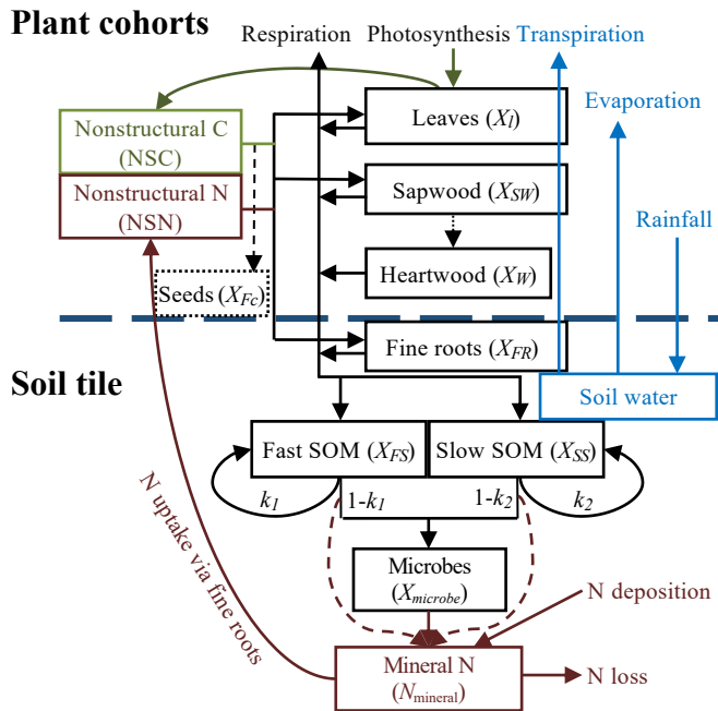
(b) Biogeochemical structure
