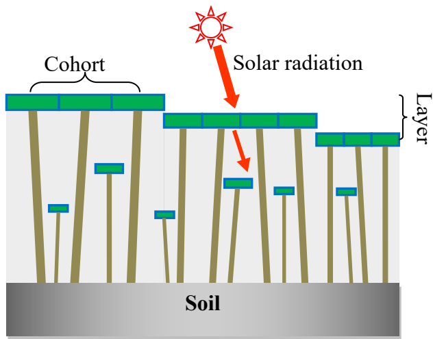
(a) Community structure
