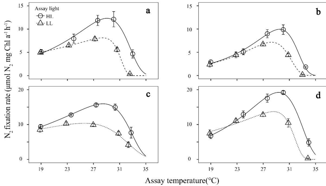
Figure S2. Short-term temperature norms of N 2 fixation measured at two light intensity (HL: 160 μmol quanta m -2 s -1 , LL: 50 μmol quanta m -2 s -1 ) in Trichodesmium acclimated to: (a) 23 °C and LL, (b) 27°C and LL, (c) 23°C and HL, (d) 27°C and HL. Values represent the means ± standard deviations of biological replicates (n=3). Fitted lines are based on mean parameters at each treatment across replicates (n=3) derived from non-linear least squares regression using the modified Sharpe-Schoolfield model (function ‘nlm’ in package ‘stats’ in R).
