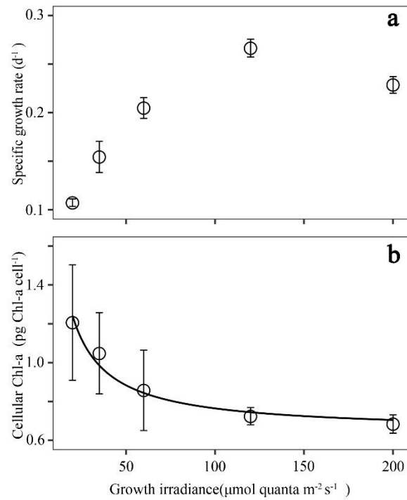
Figure S1. (a) Specific growth rate and (b) cellular Chl-a content of Trichodesmium grown across a range of light intensity. Values represent the means \pm standard deviations of biological replicates (n=3). Cultures were grown at 25°C without aeration. In panel (b), the curve gives the best fit using inverse proportional function: y = 11.9233x + 0.6451 .
