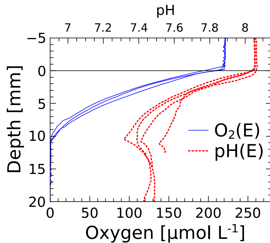
(c) Distal
