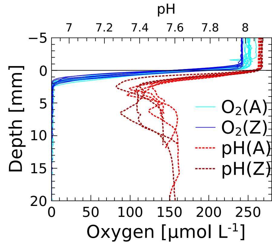
(a) Proximal
