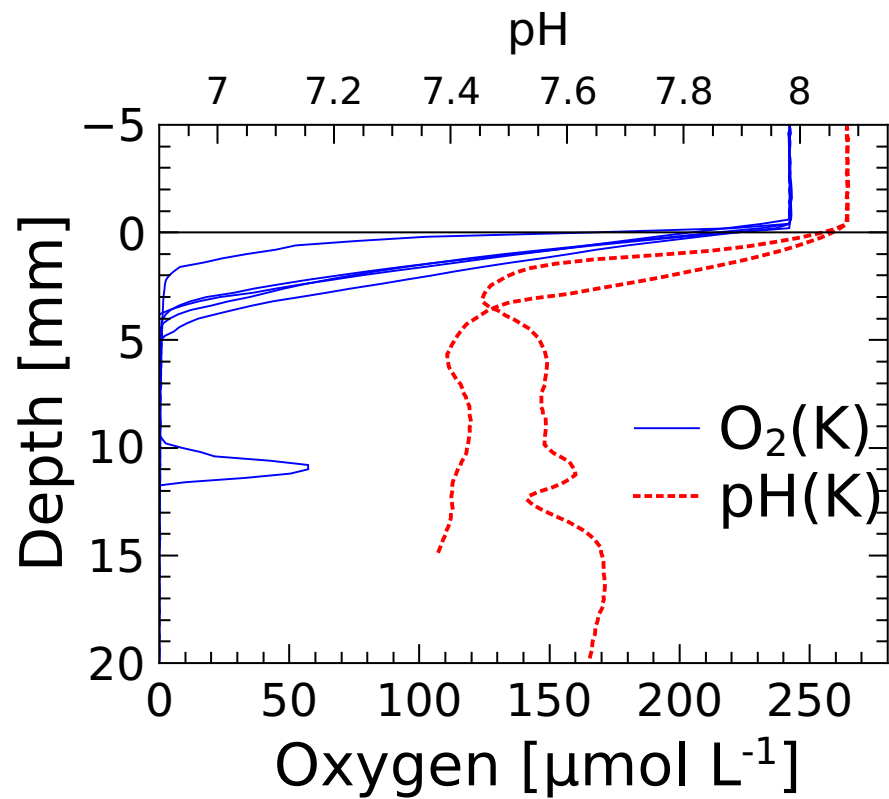
(b) Prodelta
