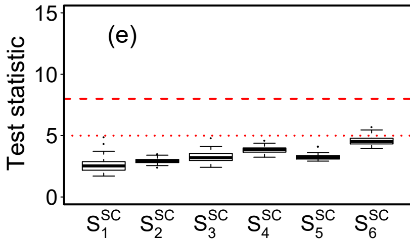
Kurtosis
