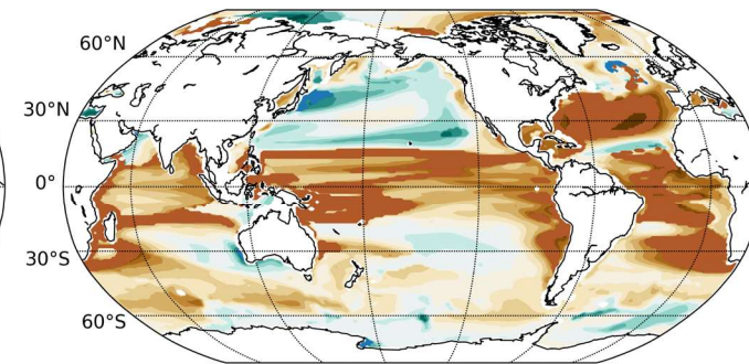
(i) CESM1.0
