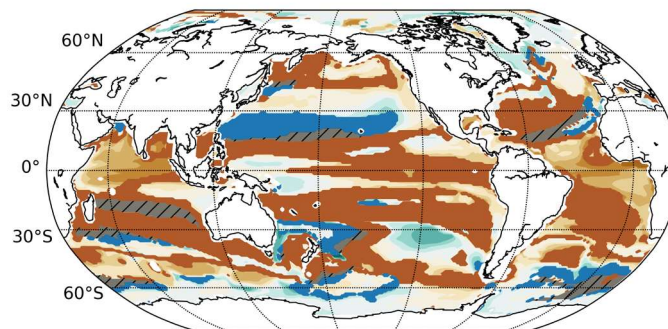
(e) IPSL-CM5A-MR
