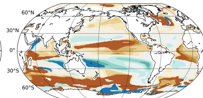
(f) IPSL-CM5A-LR
