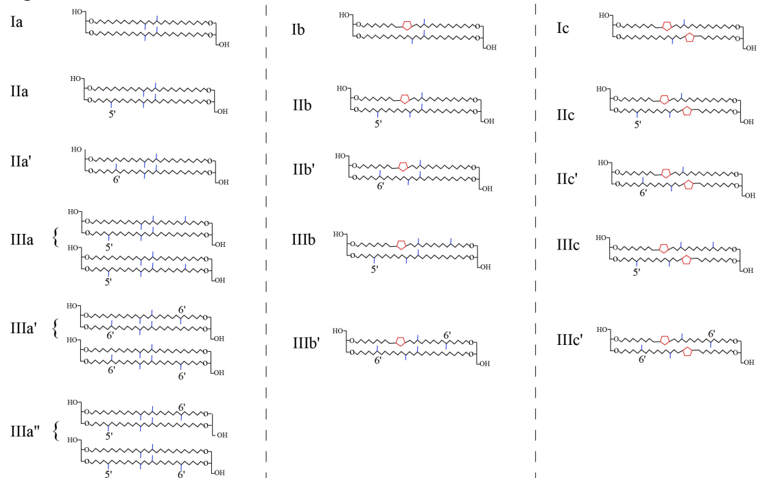
Fig. S1 Molecular structures of brGDGTs
