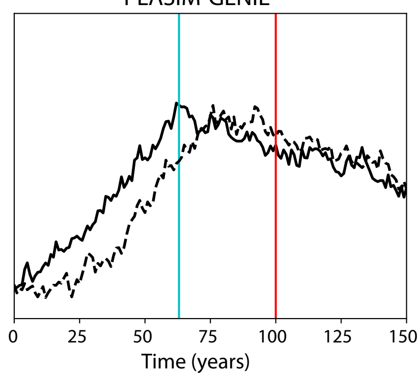
PLASIM-GENIE
