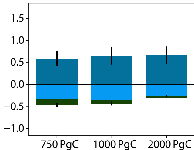
Bern3D-LPX
