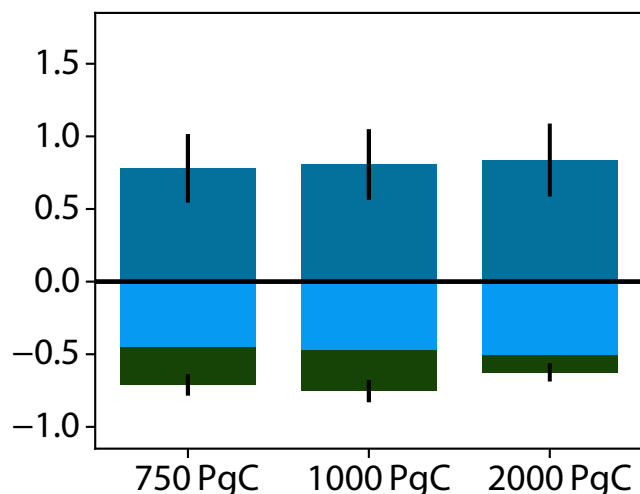
MIROC-lite
