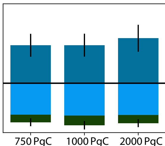
PLASIM-GENIE
