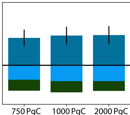
PLASIM-GENIE
