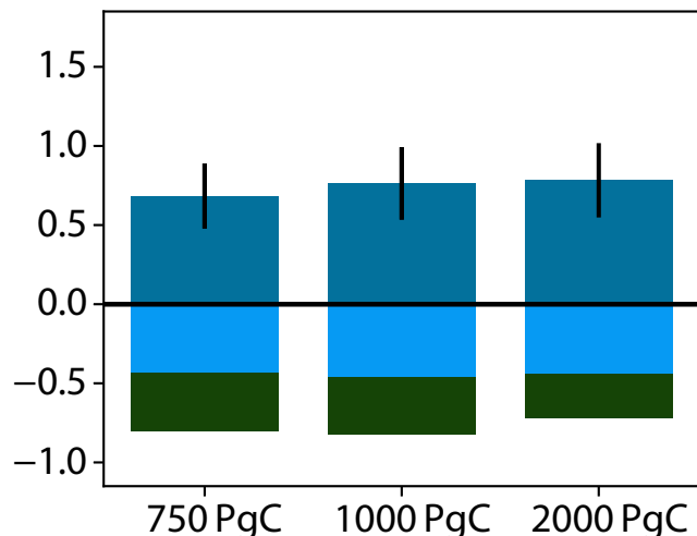
MIROC-lite
