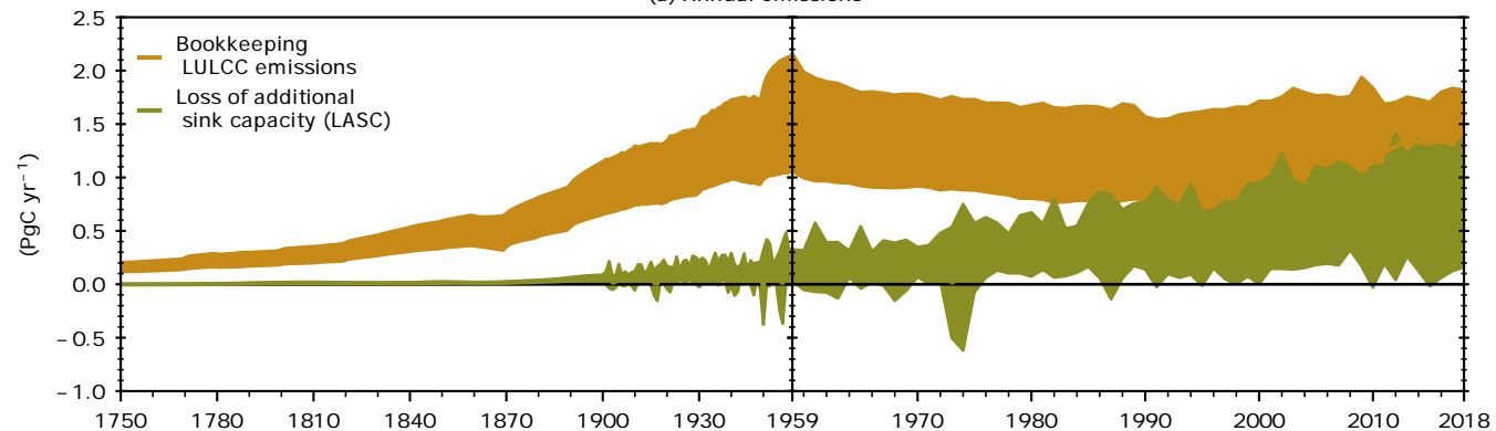
(b) Cumulative emissions
