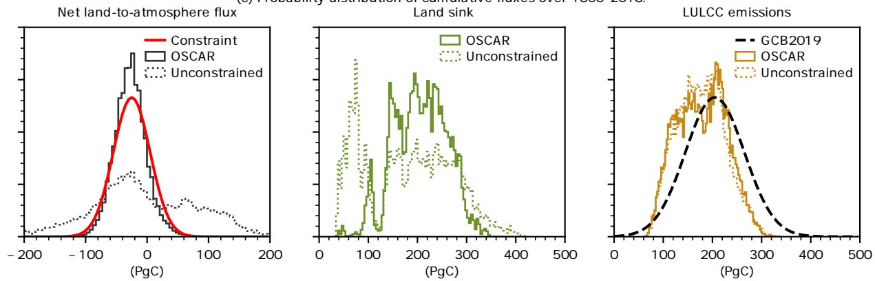
(c) Probability distribution of cumulative fluxes over 1850–2018:
