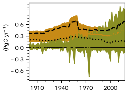
7: Wood harvest
