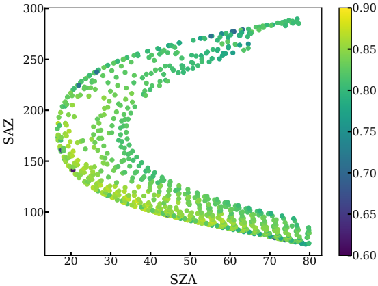
Pine NDVI
