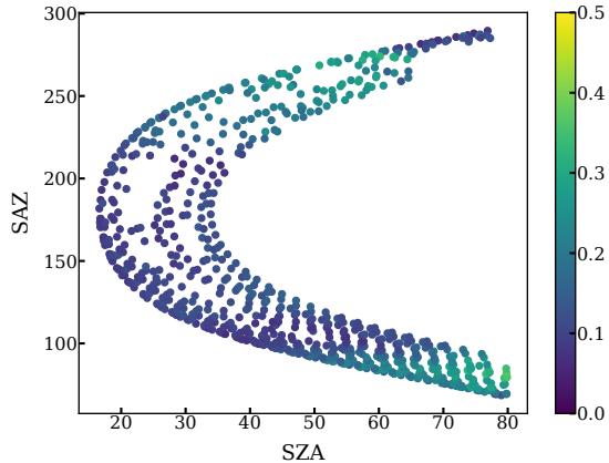
Pine NIRv
