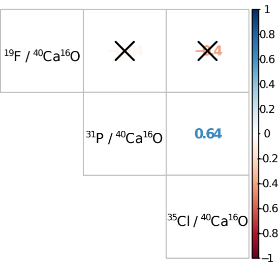
Archaias angulatus , n=46
