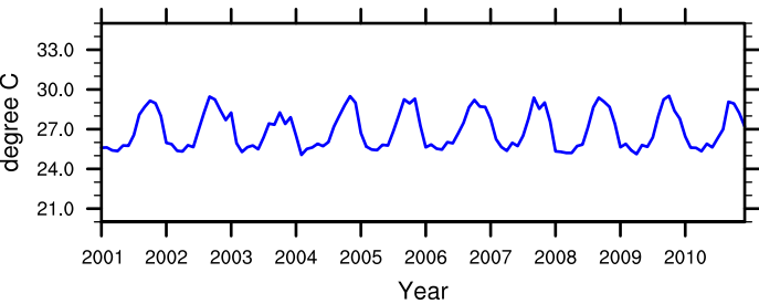
(k) 10 cm soil temperature (intact)
