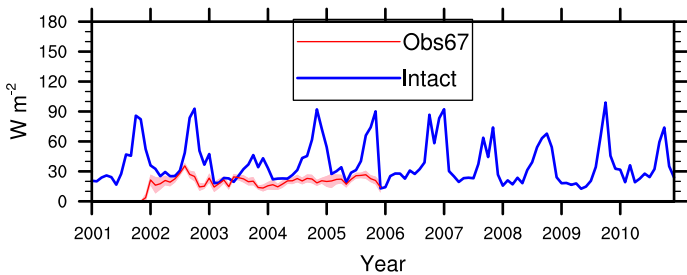
(c) Latent heat flux (intact)
