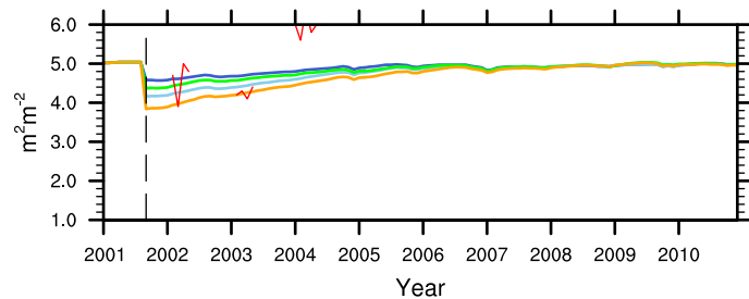
(h) Soil water in top 10 cm (logged)
