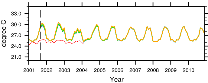
(l) 10 cm soil temperature (logged)
