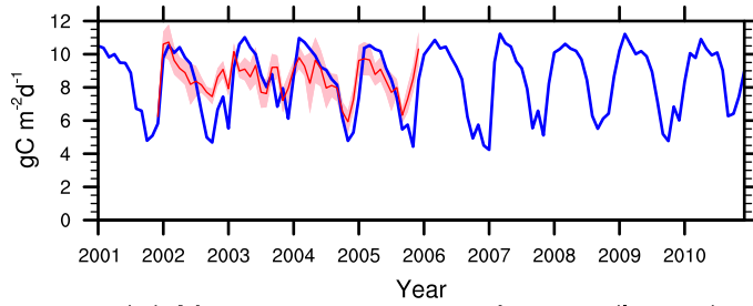
(e) Net ecosystem exchange (intact)
