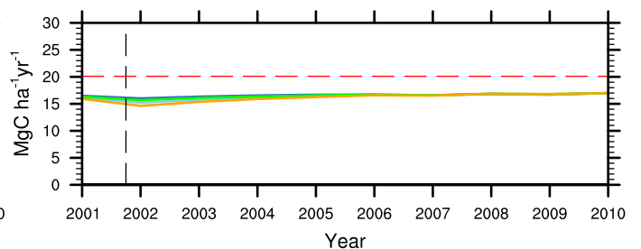
(l) Autotrophic respiration (logged)
