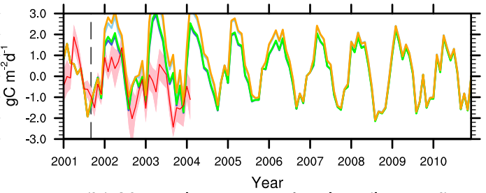
(h) Net primary production (logged)
