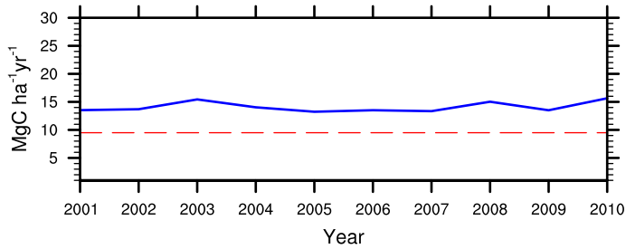
(i) Heterotrophic respiration (intact)
