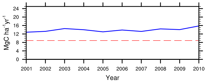
(k) Autotrophic respiration (intact)
