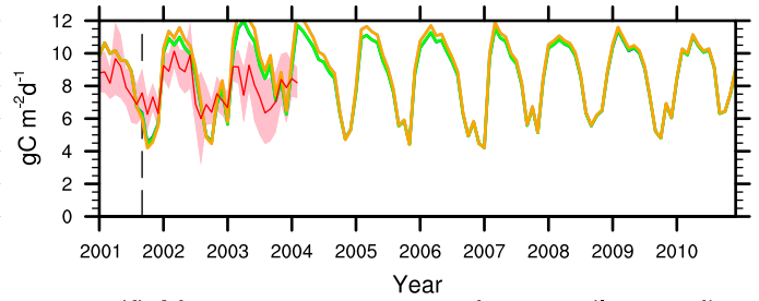
(f) Net ecosystem exchange (logged)
