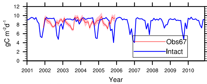
(c) Ecosystem respiration (intact)
