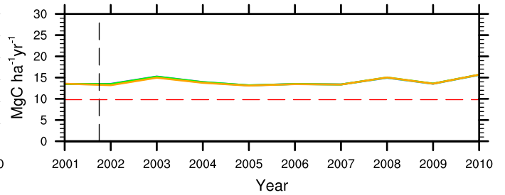
(j) Heterotrophic respiration (logged)
