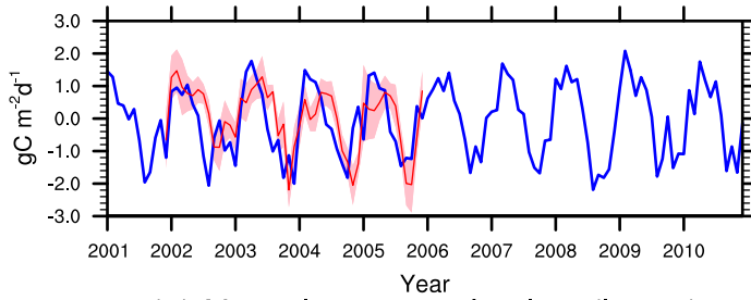
(g) Net primary production (intact)
