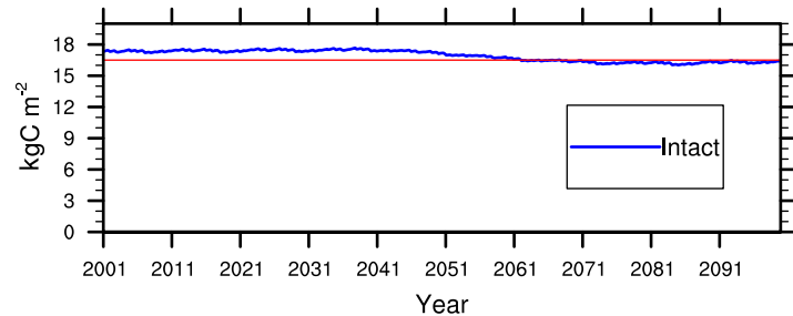
(c) Coarse woody debris (intact)
