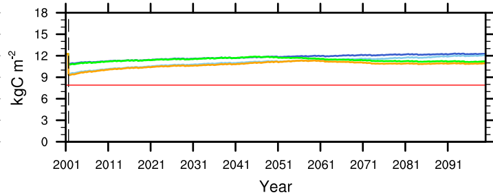
(h) Aboveground biomass, late (logged)
