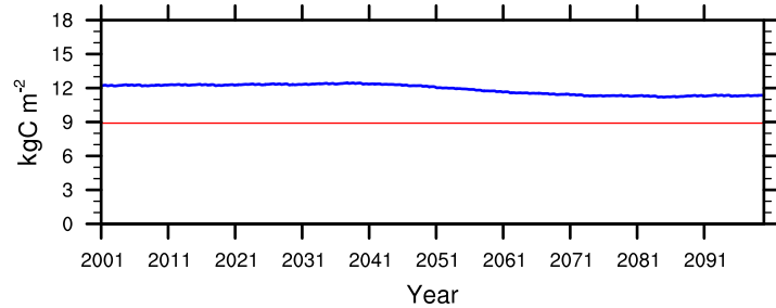
(g) Aboveground biomass, late (intact)
