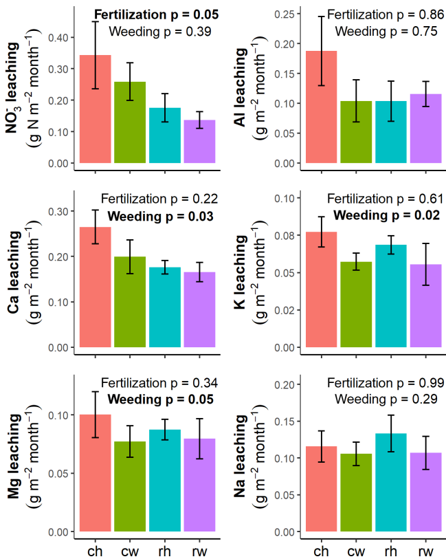
Figure 5. Average monthly leaching losses at 1.5 m depth for each experimental treatment from March 2017 to February 2018 (means \pm standard errors, n = 4 plots). Effects of fertilization and weeding were evaluated using linear mixed effects models with monthly sampling as the random effect and plots nested by management zone with subplot as the random effect; there was no significant effect of fertilization and weeding interaction. Treatments: ch is conventional fertilization–herbicide, cw is conventional fertilization–mechanical weeding, rh is reduced fertilization–herbicide, and rw is reduced fertilization–mechanical weeding.
