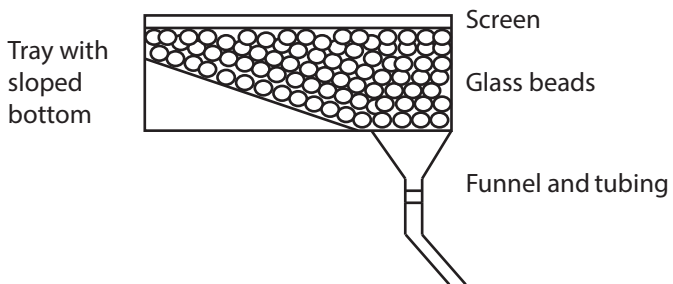
(b) Lysimeter design
