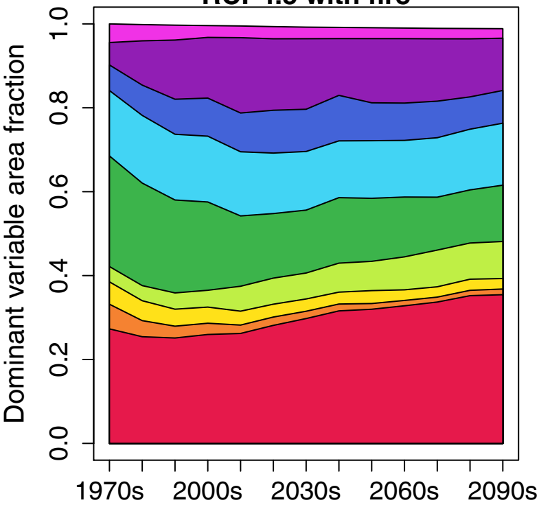
RCP4.5 with fire
