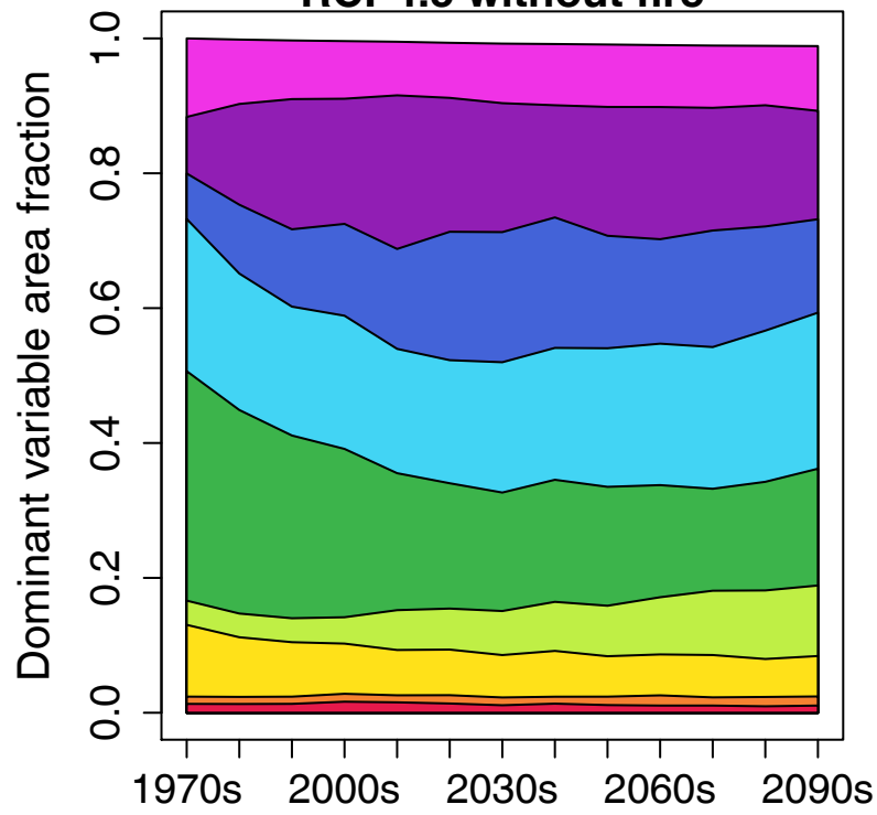
RCP4.5 without fire
