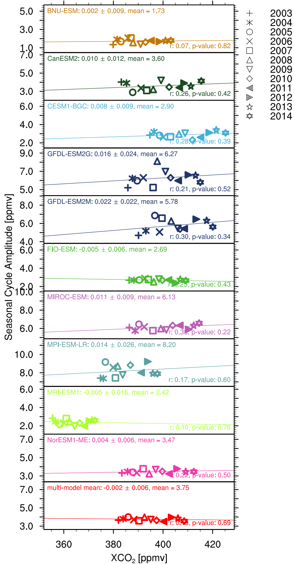
(b) GOSAT mask
