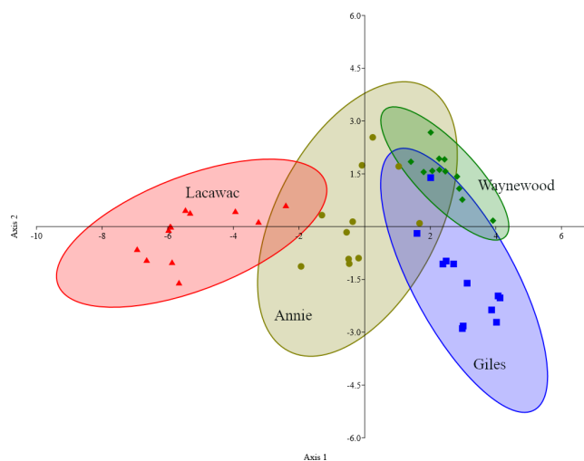
Figure 3. Canonical plot scores and 95 % confidence ellipses from descriptive discriminant analysis of the measured changes (i.e., treatment minus control) in the five variables (DOC, DIC, DO, \text{SUVA}_{320} , and S_r ) and four lakes, namely Annie (olive circles), Giles (blue squares), Lacawac (red triangles), and Wayneewood (green diamonds). Only photodegradation samples were included in this analysis.
