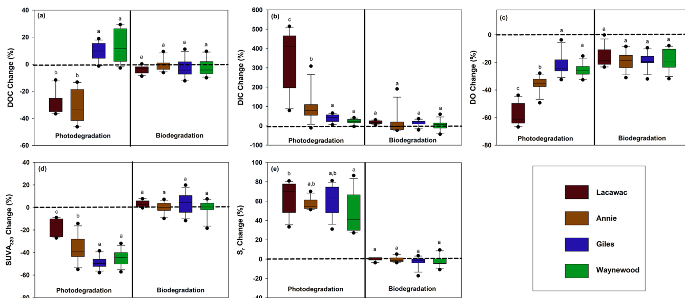
Figure 1. The monthly average percent change from the dark and killed control treatments (dashed line) in each lake for photodegradation (left) and biodegradation (right) for (a) DOC, (b) DIC, (c) DO, (d) SUVA 320 , and (e) S_r . Statistical differences ( p < 0.05 ) between the lakes are indicated by different letters above each box plot. For each box plot, n = 12 replicates.
