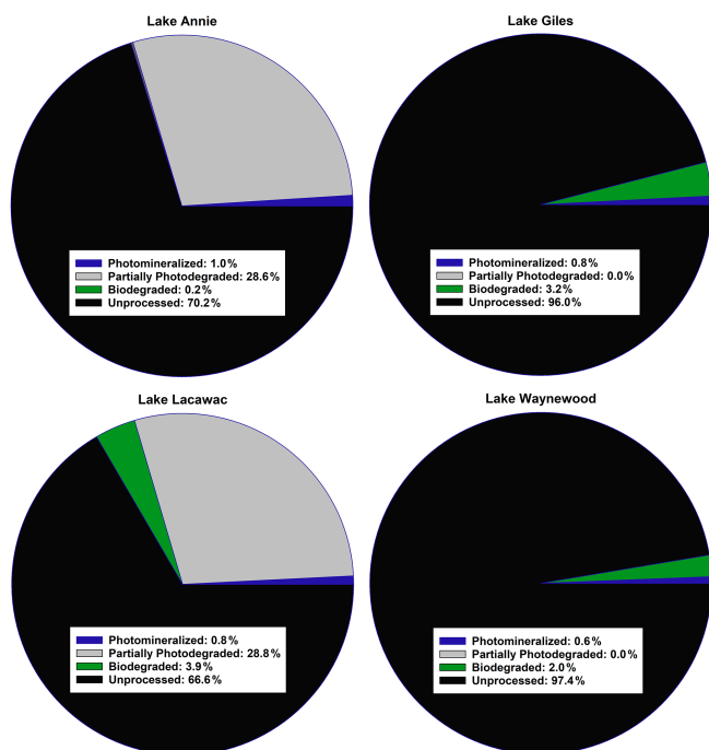
Figure 2. A summary of the average fate of carbon in the groundwater samples from our study lakes (see Sect. 2 for an explanation of the calculations). All terms were converted to a carbon basis. Photomineralized describes the amount of carbon completely mineralized to \text{CO}_2 by sunlight. Partially photodegraded describes the amount of carbon processed by sunlight minus the amount photomineralized. Biodegraded describes the amount of carbon lost through biodegradation. Unprocessed carbon describes the remaining carbon that was not processed by photodegradation or biodegradation.
