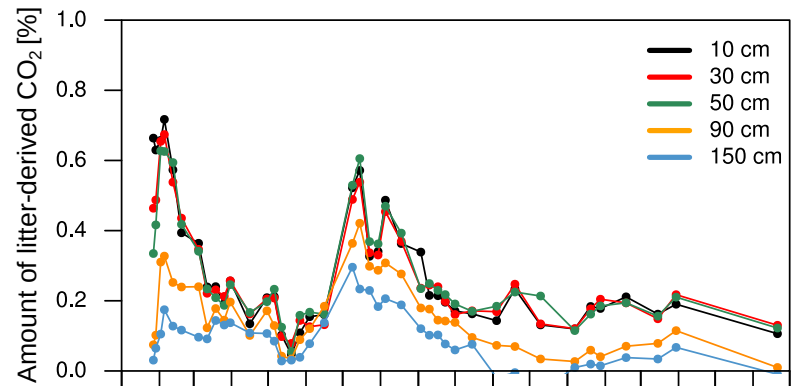
(c) Litter-derived C in CO 2
