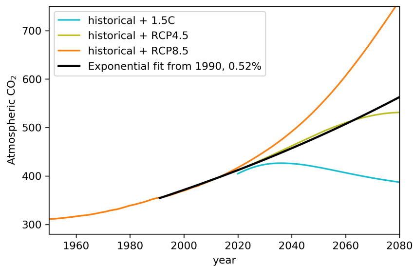
Figure S3. Comparison of scenario pCO_2^{atm} to exponential fit from 1990: 1.5°C (cyan), RCP4.5 (olive), RCP8.5 (orange), pCO_2^{atm}(\text{year}) = pCO_2^{atm}(1990) * e^{0.0052 * (\text{year} - 1990)} (black).
