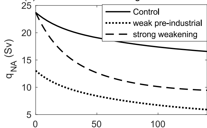
(b) Meridional Overturning
