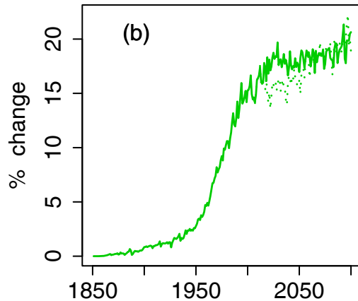
NO 3 leaching
