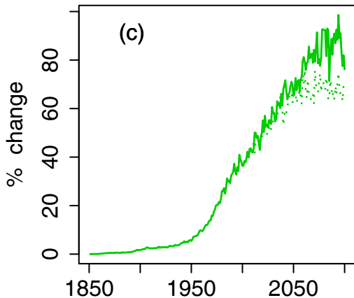
NH 4 leaching
