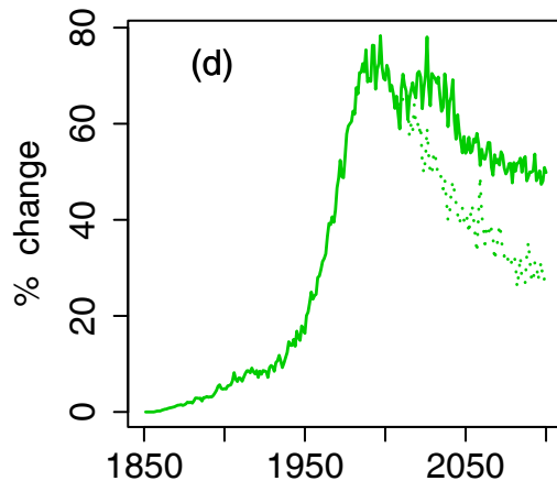
NO 3 leaching
