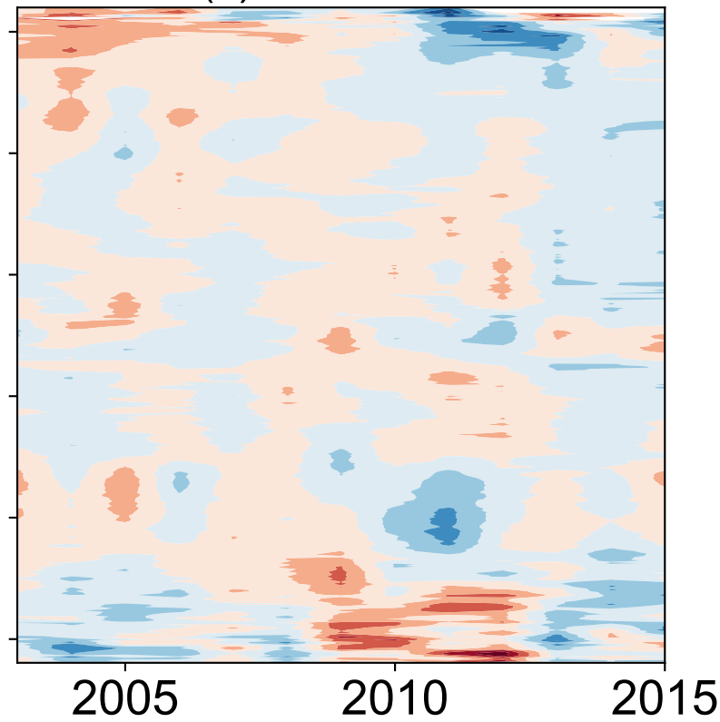
(c) GPPmodis
