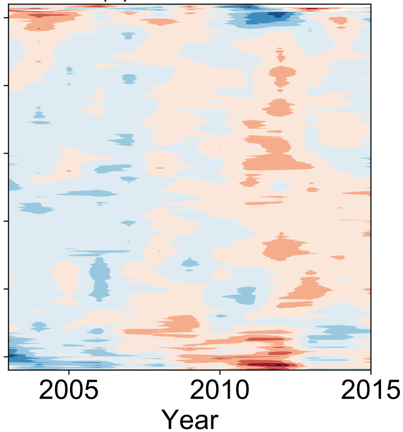
(b) GPPfluxcom
