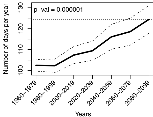
(c) PFT-MC under RCP 8.5
