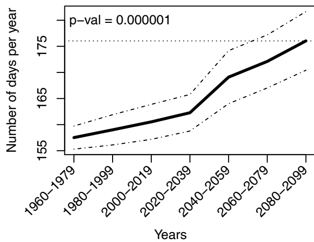
(e) PFT-HA under RCP 8.5
