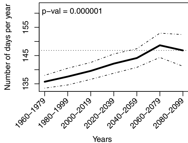
(b) PFT-LA under RCP 4.5
