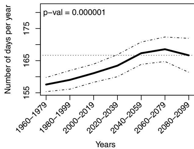
(f) PFT-HA under RCP 4.5
