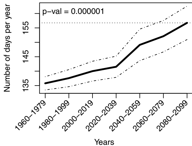
(a) PFT-LA under RCP 8.5
