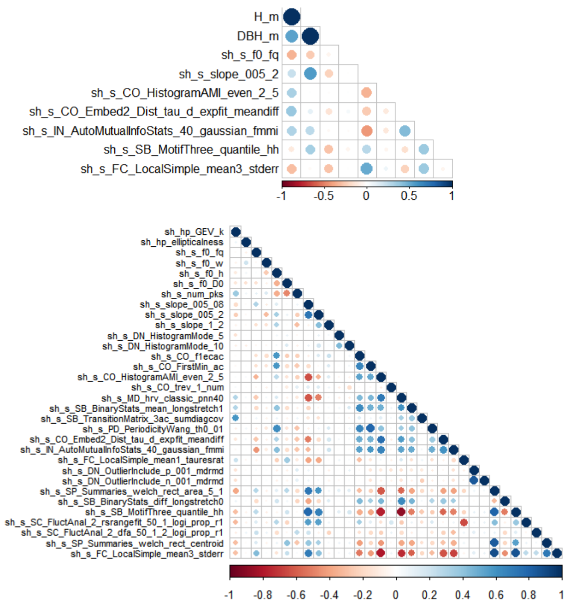
120 Figure S8 – Correlation plot for the tree motion features. Top panel shows tree height and diameter and only those features which are strongly correlated with them ( R^2 > 0.3 ). Bottom panels show all features used in this study. Colours represent strength of correlation as determined by the coefficient of determination ( R^2 )
