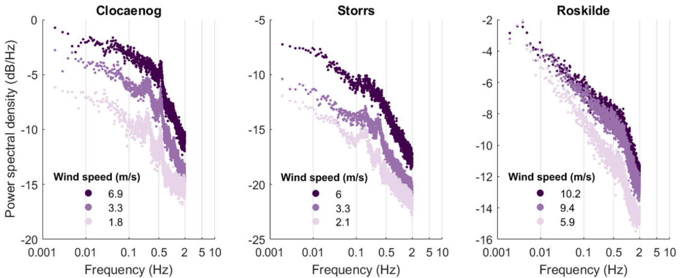
Figure S1 - Power spectra for example forest conifer (left), forest broadleaf (middle) and open-grown broadleaf (right) in high medium and low wind speeds (colours).
