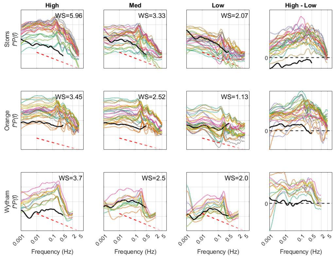
100 Figure S6 – power spectra for hourly samples of tree motion data (coloured lines) and wind speeds (black lines) at high, medium and low wind speed. Y-axis labels are the site names. The y-axis can be thought of as a measure of the relative energy content, in arbitrary units. The red dashed lines show the -2/3 slope as a reference point. The right-hand panels shows the difference between high and low wind speeds and the horizontal dashed line represents 0 change. Numbers in the top right-hand corners show the mean hourly wind speeds for the data sample. All of these sites are forest broadleaf trees.
