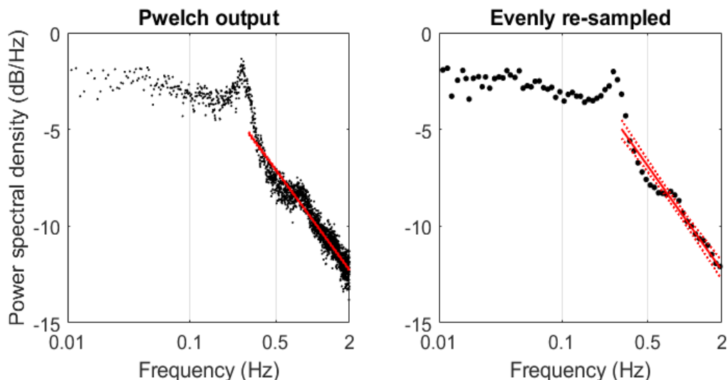
65 Figure S2 - Linear models of the power spectra to calculate slope using output of pwelch directly (left) and logarithmically re-sampled output (right). The frequency interval used in the above is 0.3 - 2 Hz.
