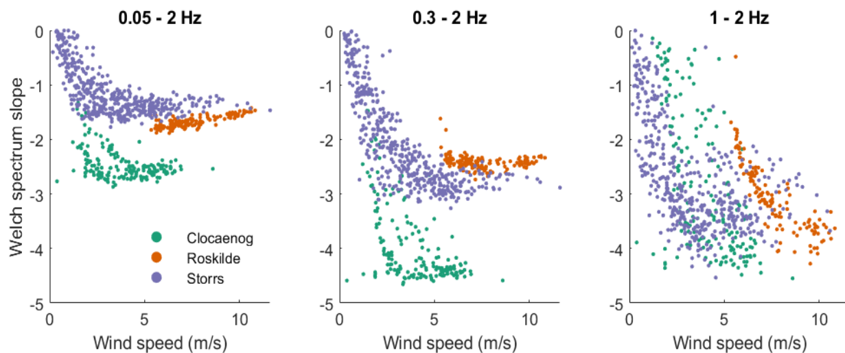
Figure S4 – Same as figure S3 but calculated using the logarithmically re-sampled power spectrum output.
