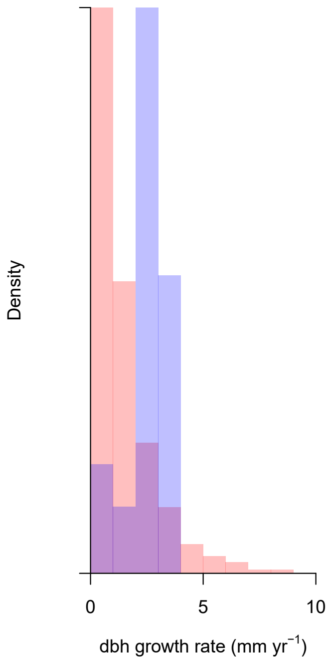
(a) Acer
