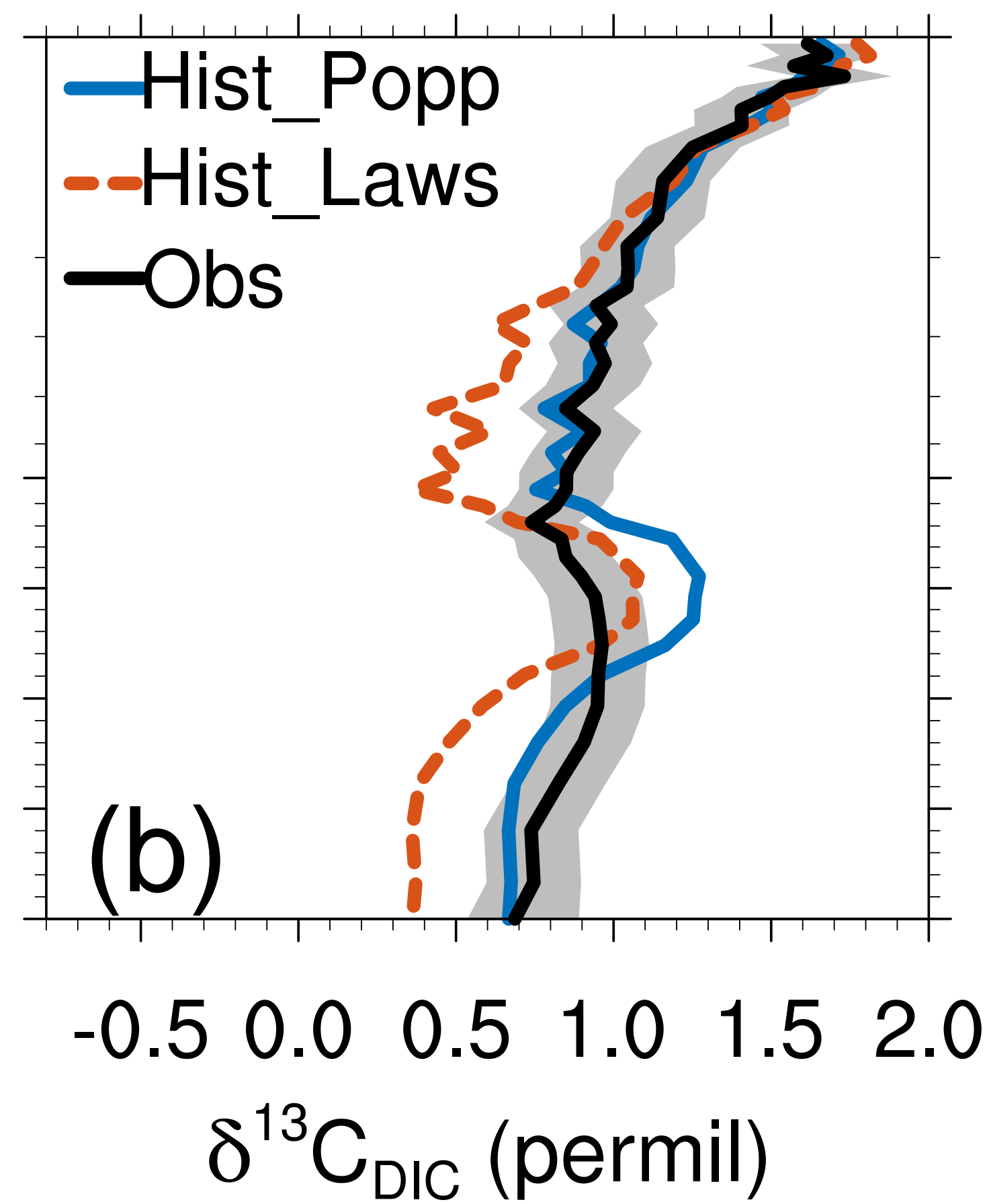
Atlantic basin-mean
