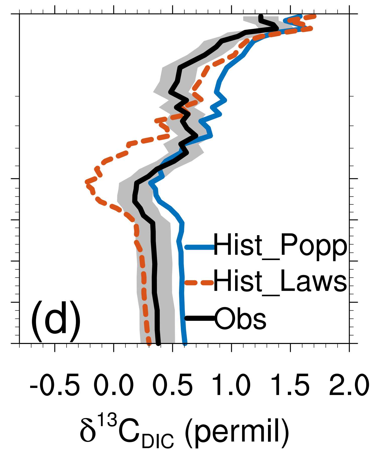
Indian basin-mean
