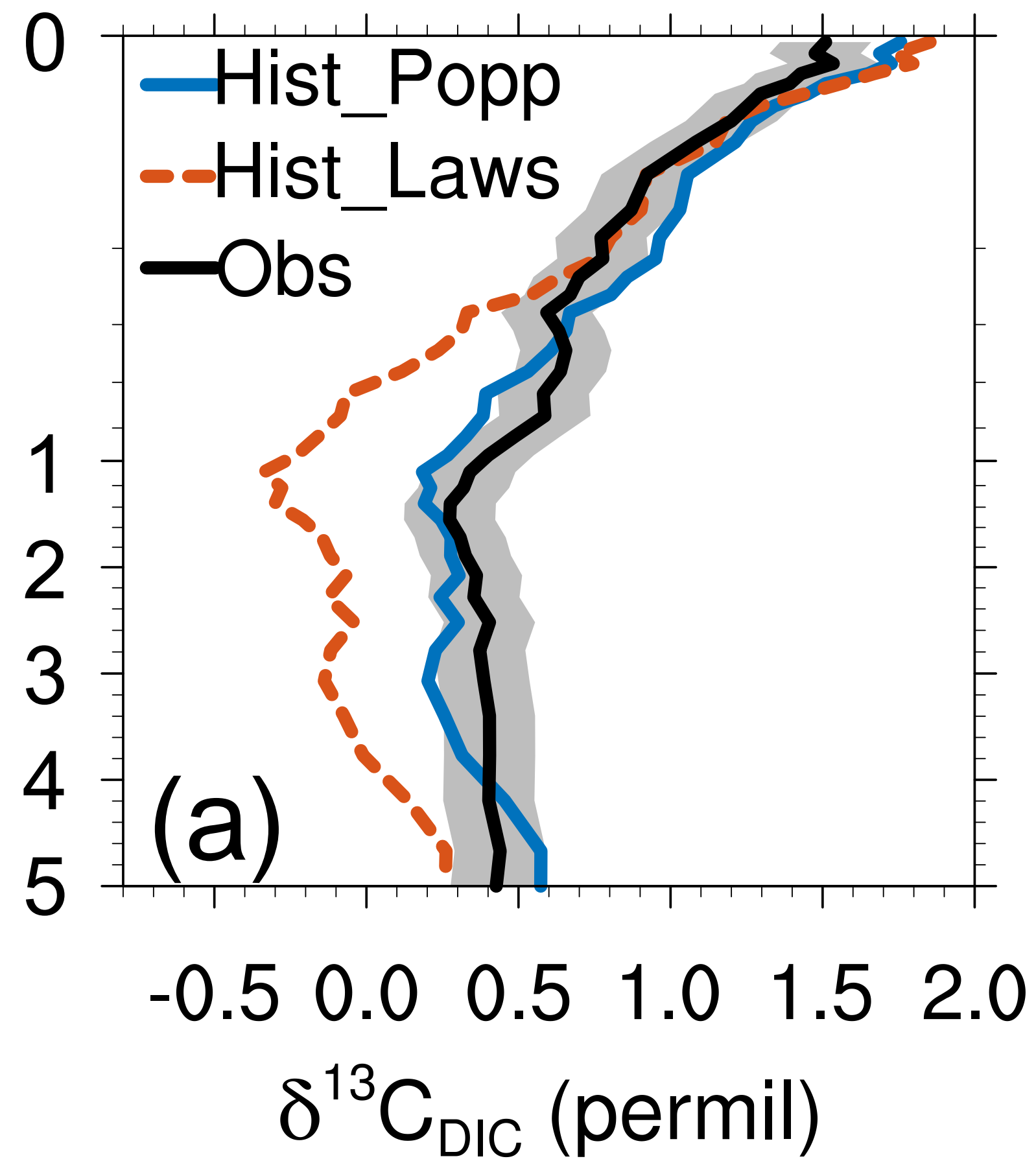
Global-mean
