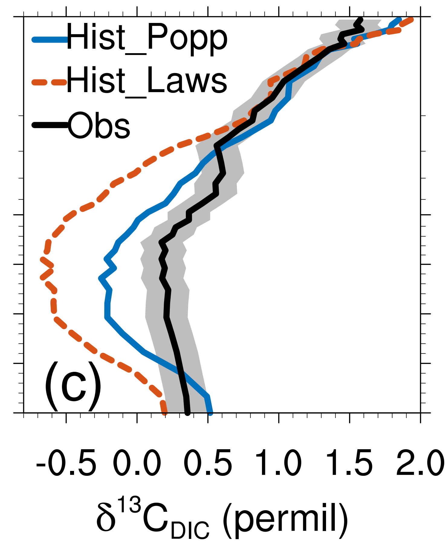
Pacific basin-mean
