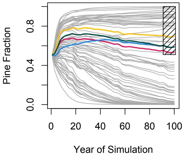
Composition with Fire On From Bare Ground
