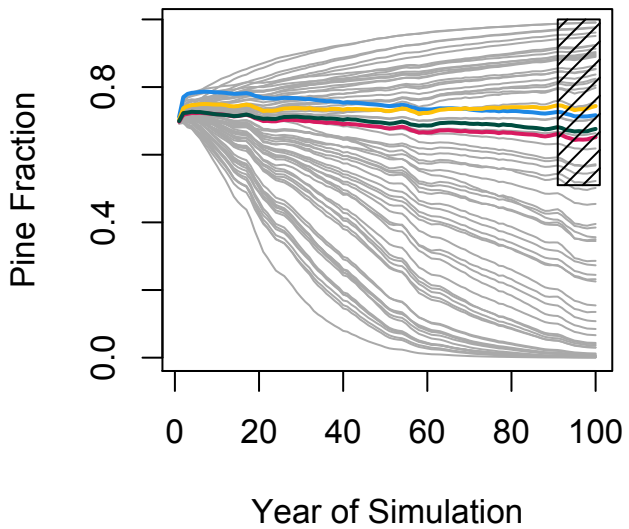
Composition with Fire On From Initialized Stands
