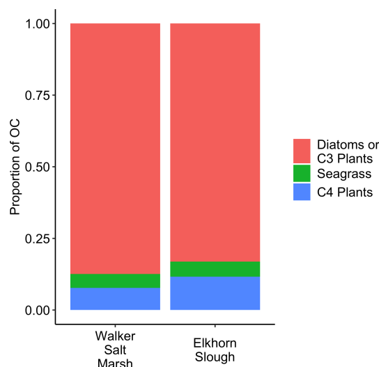
Figure 7. Mixing model results displaying the average source contributions to salt marsh sediment organic carbon (OC) for two salt marshes. Exact values and significance are shown in Table S2.
