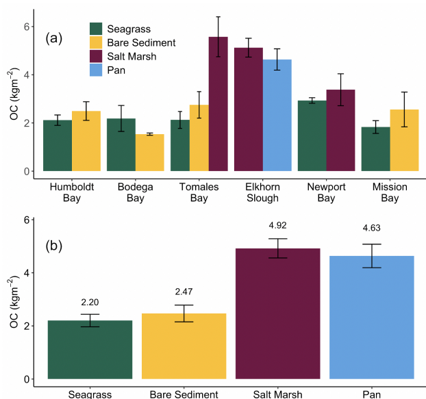
Figure 3. Average ( \pm SE) total organic carbon (OC) stocks ( \text{kg m}^{-2} ) across all cores collected from each habitat type within each site in this study (a). Average ( \pm SE) total organic carbon stocks ( \text{kg m}^{-2} ) across all cores collected within each habitat type in this study (b). Stocks are representative of the top 20 cm of sediment.
