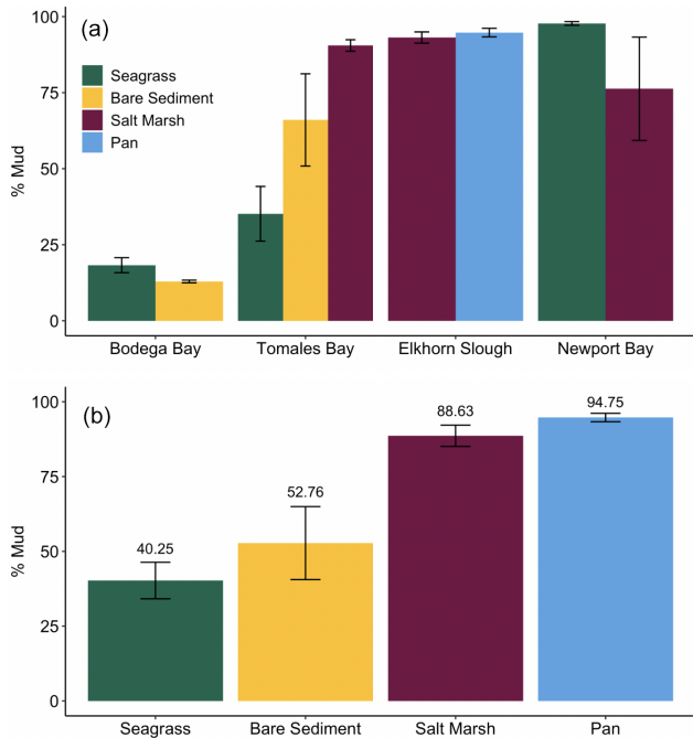
Figure 5. Average ( \pm SE) percent mud of all sediments quantified in each site within each habitat type (a), and average ( \pm SE) percent mud in each habitat type across all sites measured (b).
