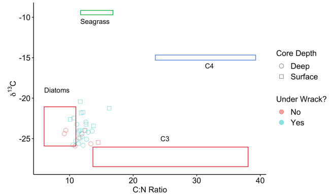
Figure 6. Points represent the \delta^{13}\text{C} and C : N ratios of Walker Salt Marsh sediment data, collected from underneath persistent wrack lines (blue) and from areas free of wrack (red) (see Fig. 1c). Sediment subsamples collected from the surface to 10 cm deep are labeled as surface samples (square) and below 10 cm are labeled as deep samples (circle). Colored boxes represent sources (means \pm SD) from diatoms (red), seagrass (green), C 4 salt marsh plants (blue), and C 3 salt marsh plants (red).
