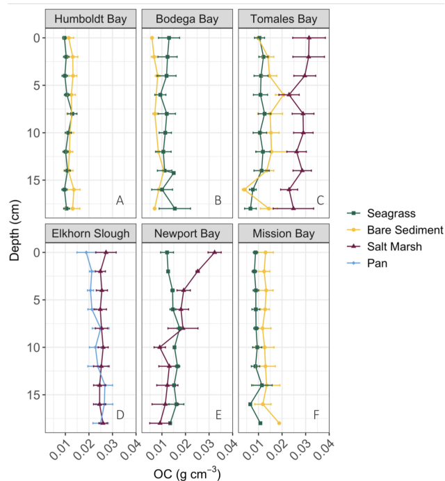
Figure 2. Down core trends (surface = 0 cm) in average ( \pm SE) OC ( \text{g cm}^{-3} ) for each habitat type and site. Data show an insignificant decline in OC through time (downcore) in all sites except Newport Bay salt marshes.
