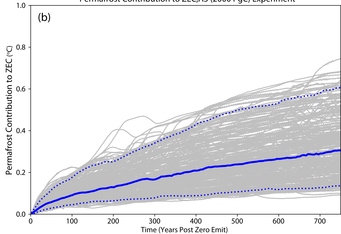
Permafrost Contribution to ZEC, A3 (2000 PgC) Experiment
