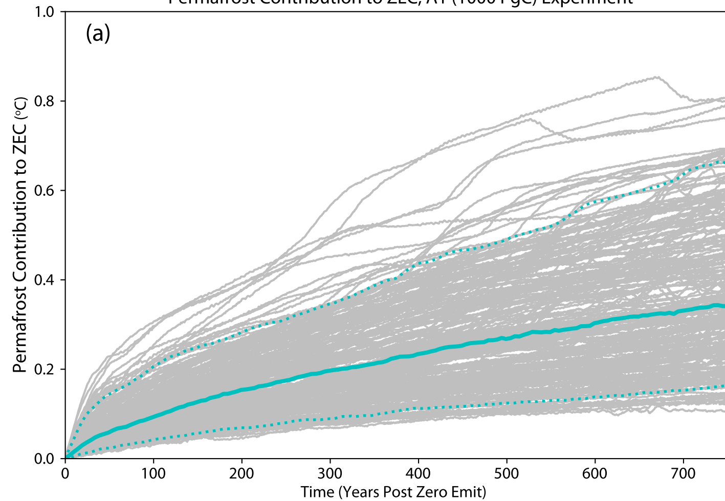
Permafrost Contribution to ZEC, A1 (1000 PgC) Experiment
