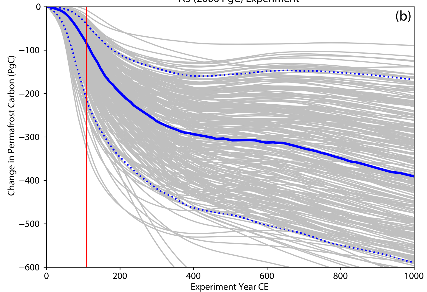
A3 (2000 PgC) Experiment
