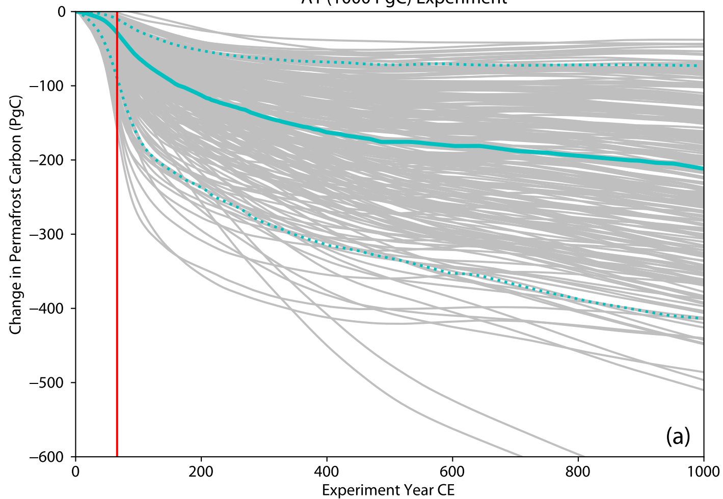
A1 (1000 PgC) Experiment
