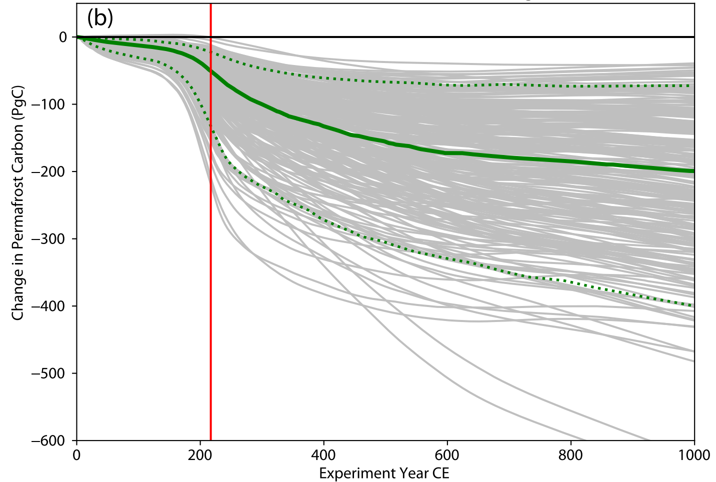
Permafrost Carbon Change
