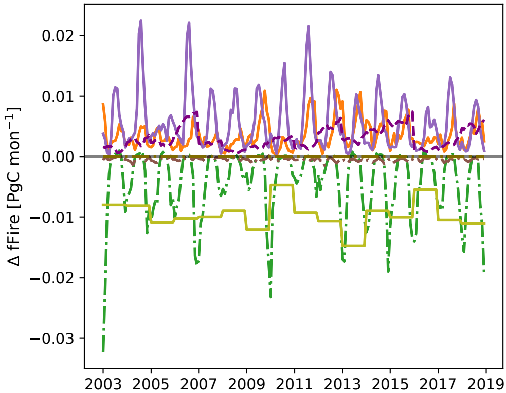
(a) Monthly fire CO 2 emissions
