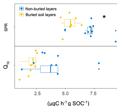
Figure 4. Boxplot of soil potential respiration (SPR) rates and SOC temperature sensitivity ( Q_{10} ). The * signifies differences in SPR or Q_{10} between the buried and non-buried soil layers ( P < 0.05 ). Identification of buried soil layers is based on the depth profile of SOC concentration and soil chemical weathering degree with support from the stretch map in Fig. 1 (see details in S1 in the Supplement).
