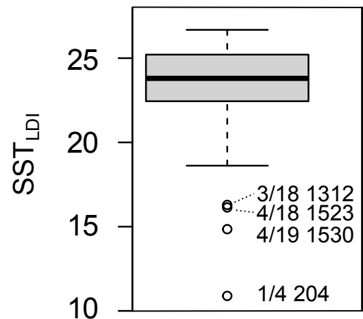
SST LDI Boxplot
