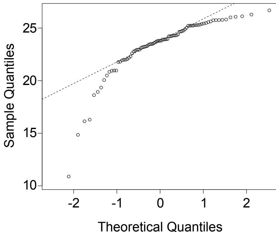
SST LDI Normal Q-Q plot
