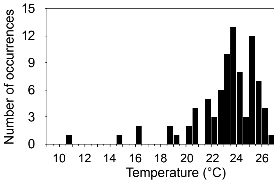
SST LDI frequency distribution
