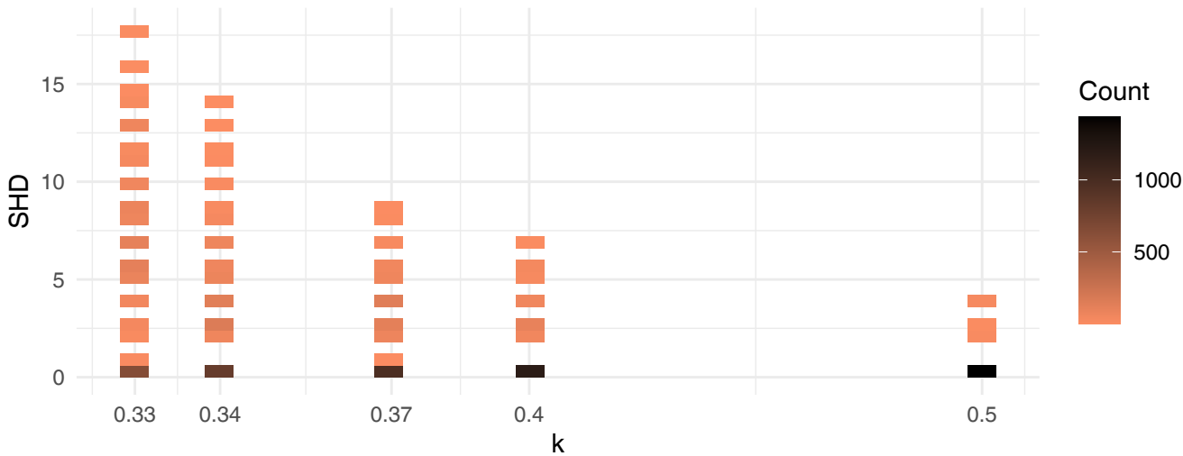
Structural Hamming distance between results from different starting points
