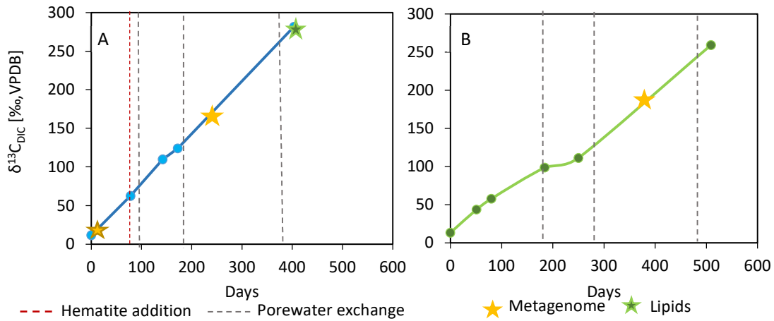
Figure S2: Change over time in the \delta^{13}\text{C}_{\text{DIC}} values of two pre-incubated slurries amended with ^{13}\text{C}\text{-CH}_4 (1.5-2 mL): (A) setup used in November 2017 with hematite addition, and (B) setup used in August 2017 without an electron acceptor addition. Sampling times for the different biological analyses (metagenome and lipids) are presented in the graphs. Black dashed lines represent the time at which 20 ml of the porewater in the bottles was exchanged with fresh porewater. The red dashed line represents the time at which hematite was added.
