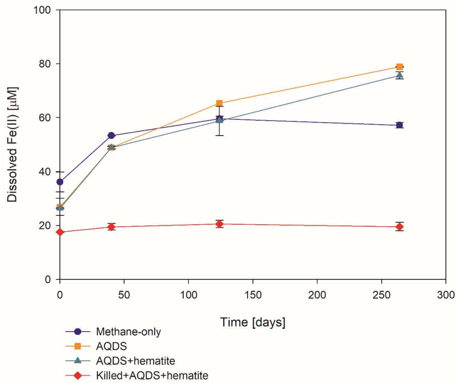
Figure S3: The change of dissolved Fe(II) in the two-stage experiment SN-6 with time. Error bars represent the average deviations of the data points from their means of duplicate/triplicate bottles.
