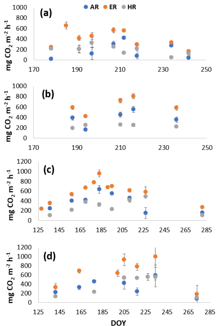
Figure A2. Average CO 2 fluxes in the (a) shrub plots and (b) sedge plots across the growing season of 2018, and CO 2 fluxes in the (c) shrub plots and (d) sedge plots across the growing season of 2019.
