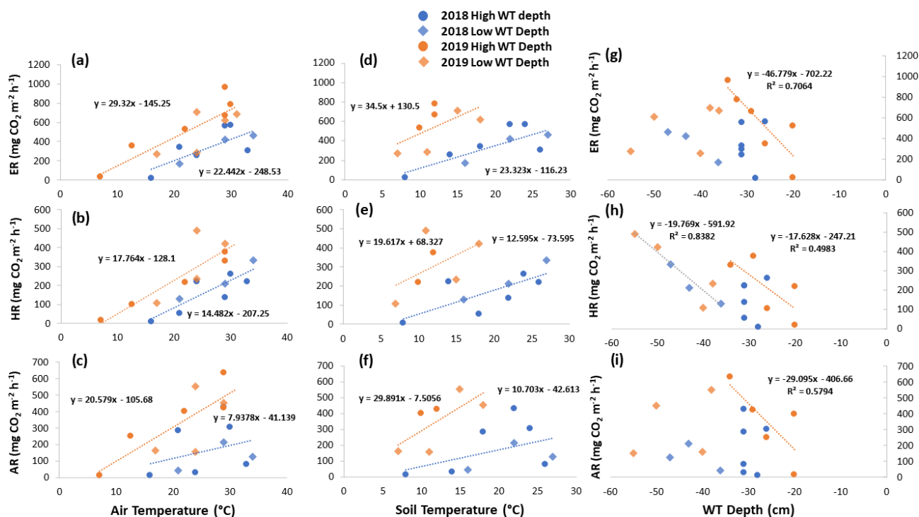
Figure 6. Scatterplots with trend lines of relationships between air temperature and (a) ER, (b) HR, and (c) AR; between soil temperature and (d) ER, (e) HR, and (f) AR; and between water table (WT) depth and (g) ER, (h) HR, and (i) AR in the shrubs across the growing seasons of 2018 and 2019. High WT refers to water table positions from surface to 35 cm depth.
