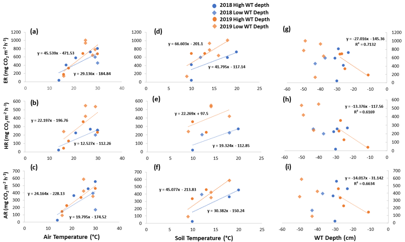
Figure 7. Scatterplots with trend lines of relationships between air temperature and (a) ER, (b) HR, and (c) AR; between soil temperature and (d) ER, (e) HR, and (f) AR; and between water table (WT) depth and (g) ER, (h) HR, and (i) AR in the sedges across the growing seasons of 2018 and 2019. High WT refers to water table positions from surface to 35 cm depth.
