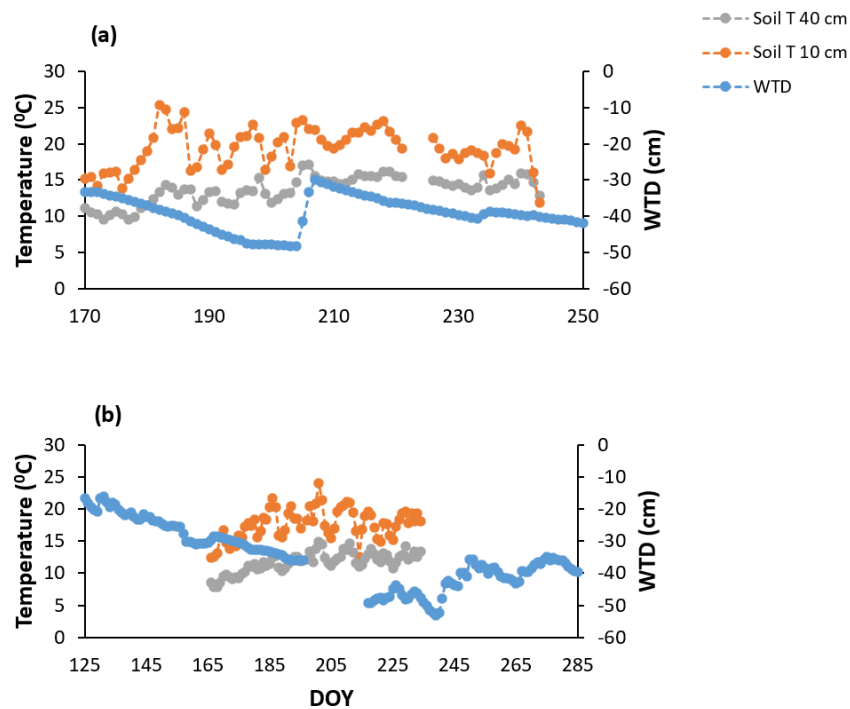
Figure A1. Continuous measures of soil temperatures (soil T ) at 10 and 40 cm and water table depth (WTD) for the growing seasons of (a) 2018 and (b) 2019 derived from the eddy covariance tower near the manual chamber setup.
