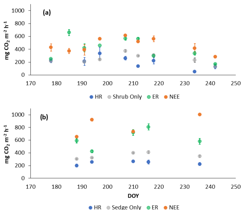
Figure 3. Average \text{CO}_2 fluxes in the (a) shrub plots and (b) sedge plots across the growing season of 2018 ( \pm standard error).
