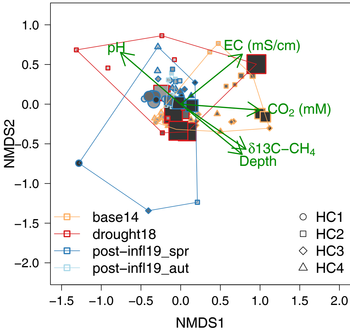
(a) Bacteria, stress = 0.15
