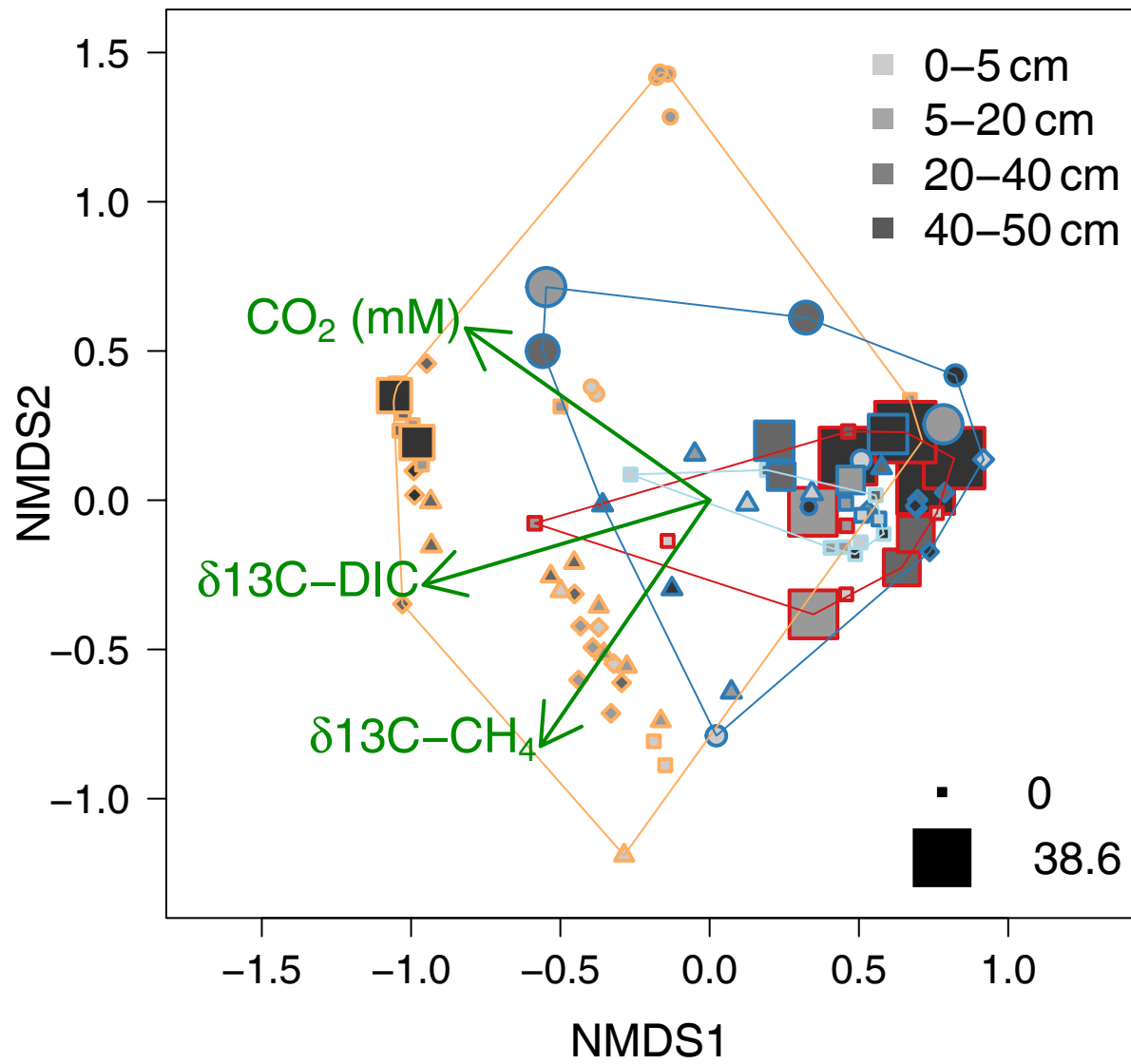
(b) Archaea, stress = 0.15
