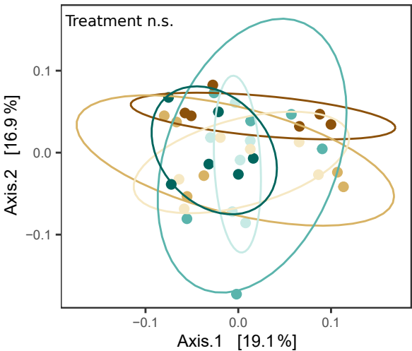
(a) Weighted UniFrac (relative abundance)
