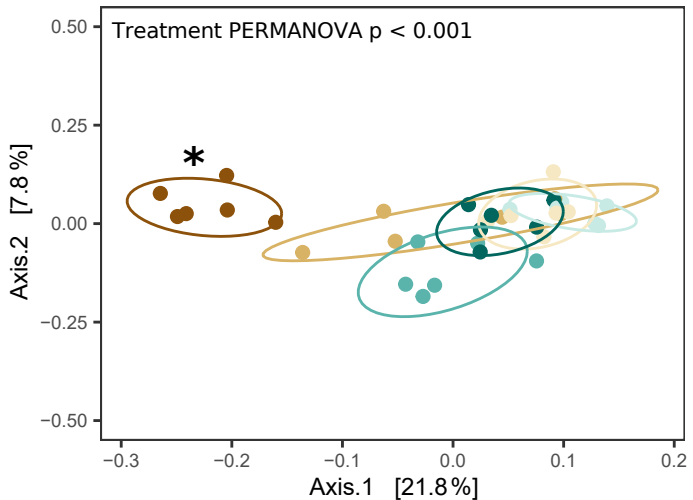
(b) Non-weighted UniFrac distance (presence-absence)
