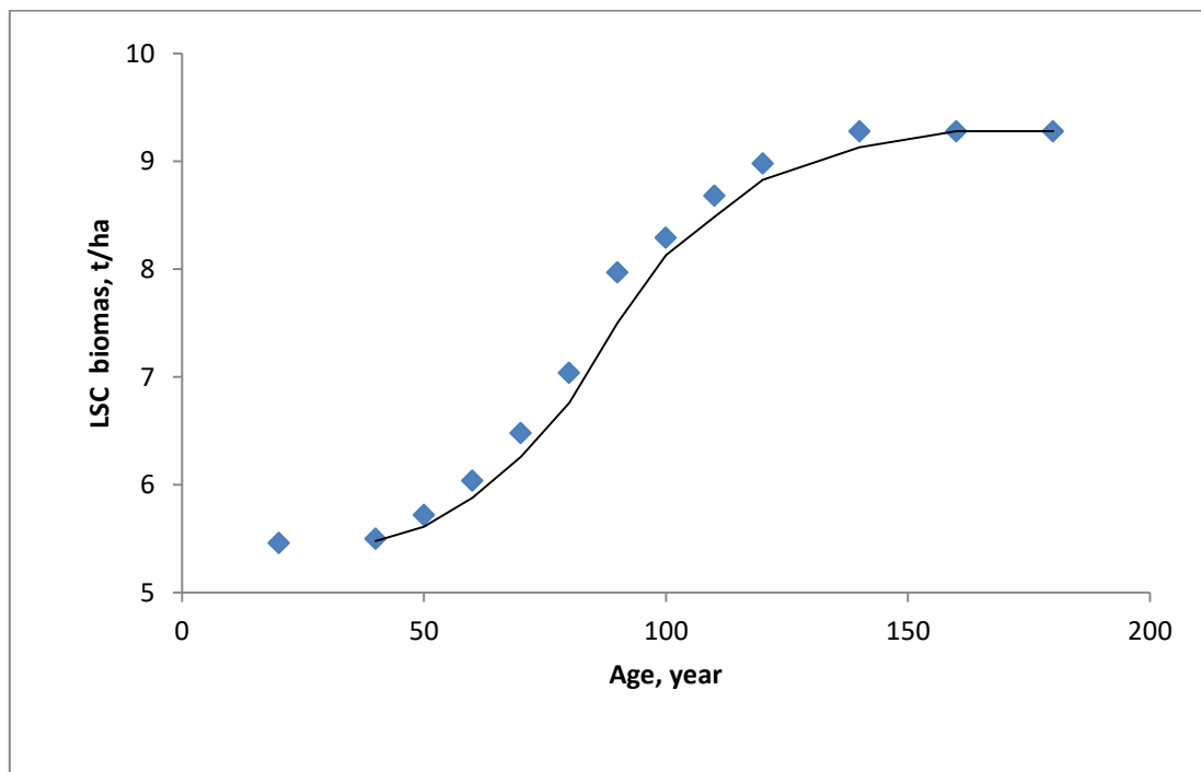
Fig. S2. Changes in the phytomass of the living soil cover (LSC) in blueberry pine forests of Karelia depending on age, after Zyabchenko (1984).
