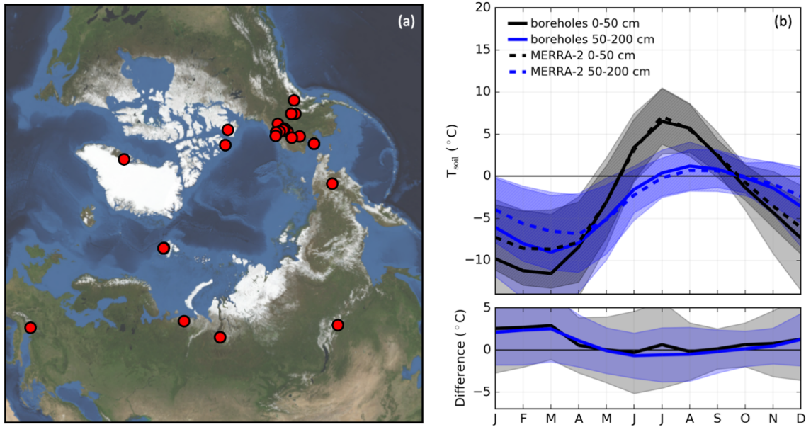
Figure S12. Comparison of MERRA-2 Land soil temperature to borehole measurements over 1998–2020. (a) locations of borehole temperature measurement sites. (b) Mean seasonal cycle of borehole temperature with shading showing one standard deviation across the sites. MERRA-2 Land soil temperatures (mean over 2015–2018) sampled at the model grids containing the boreholes.
