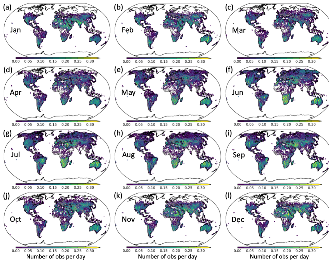
Figure S7. Spatial coverage of monthly OCO-2 land X_{CO_2} retrievals averaged over four years (2015, 2016, 2018, and 2019). (a-l) Monthly mean observations per day of OCO-2 ACOS v10 combined land nadir and land glint 10 sec X_{CO_2} super-obs on a 1^\circ \times 1^\circ spatial grid.
