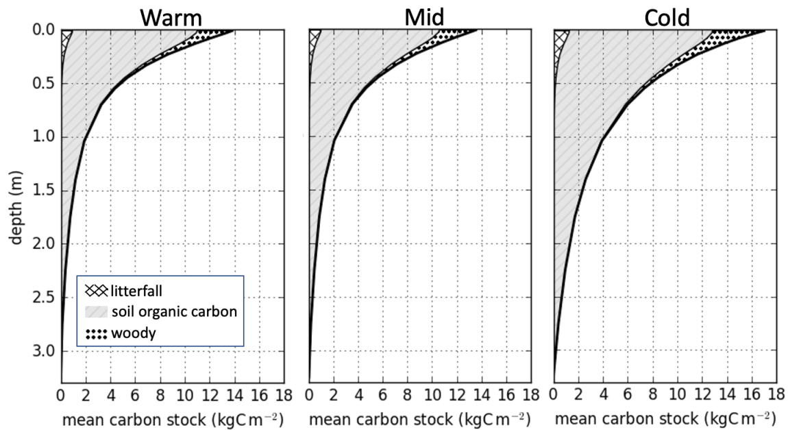
Figure S16. Regional carbon stocks with depth simulated by the soil carbon decomposition model
