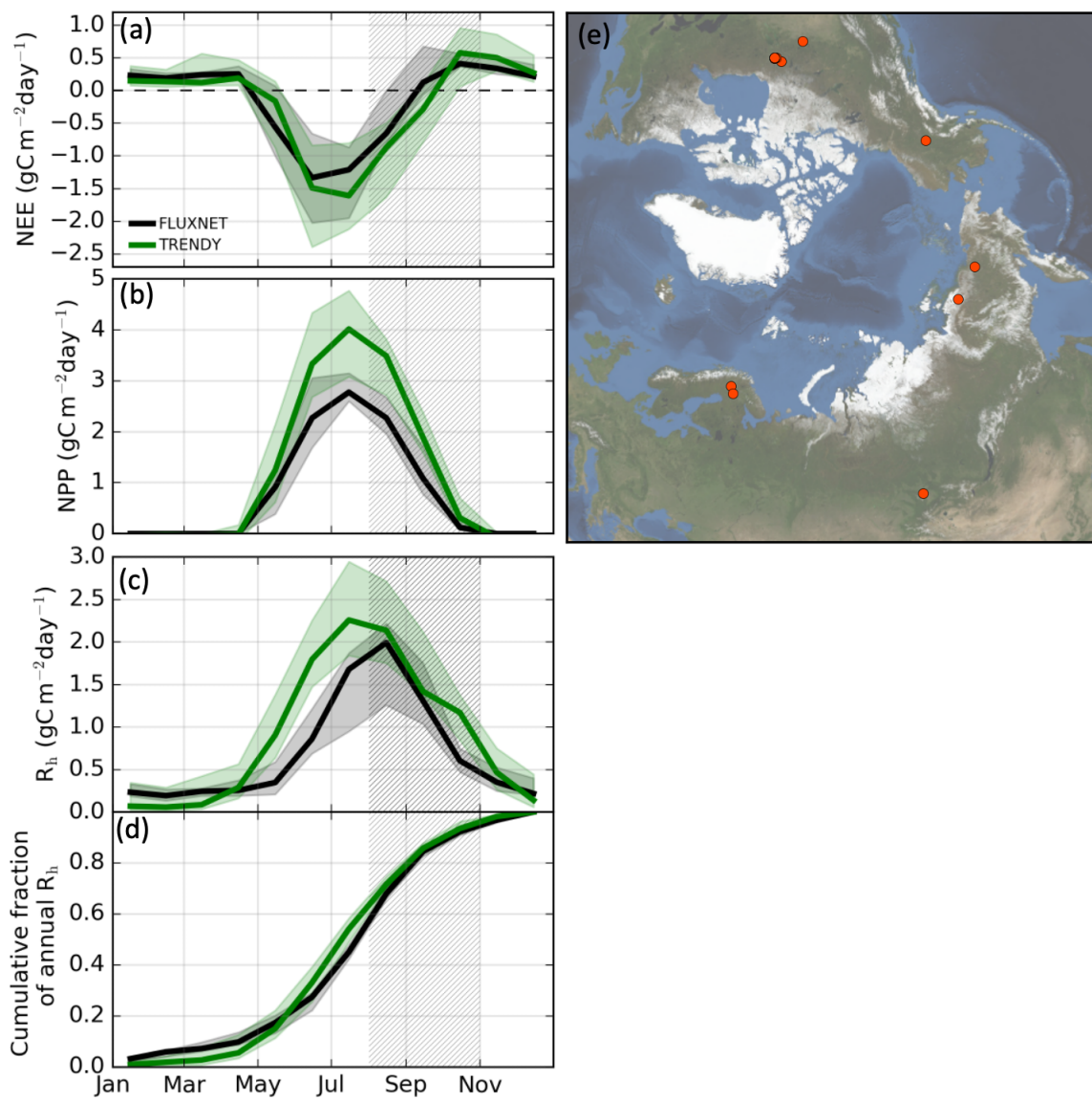
Figure S11. Median and interquartile spread in carbon fluxes measured (black) and simulated by TRENDY (green) at 15 FLUXNET sites. Mean seasonal cycles are shown for (a) NEE, (b) NPP, (c) R_h , and (d) cumulative fraction of R_h measured (black). (e) Location of 15 high-latitude FLUXNET sites in regions with the mean October air temperatures less than 2^{\circ}\text{C} .
