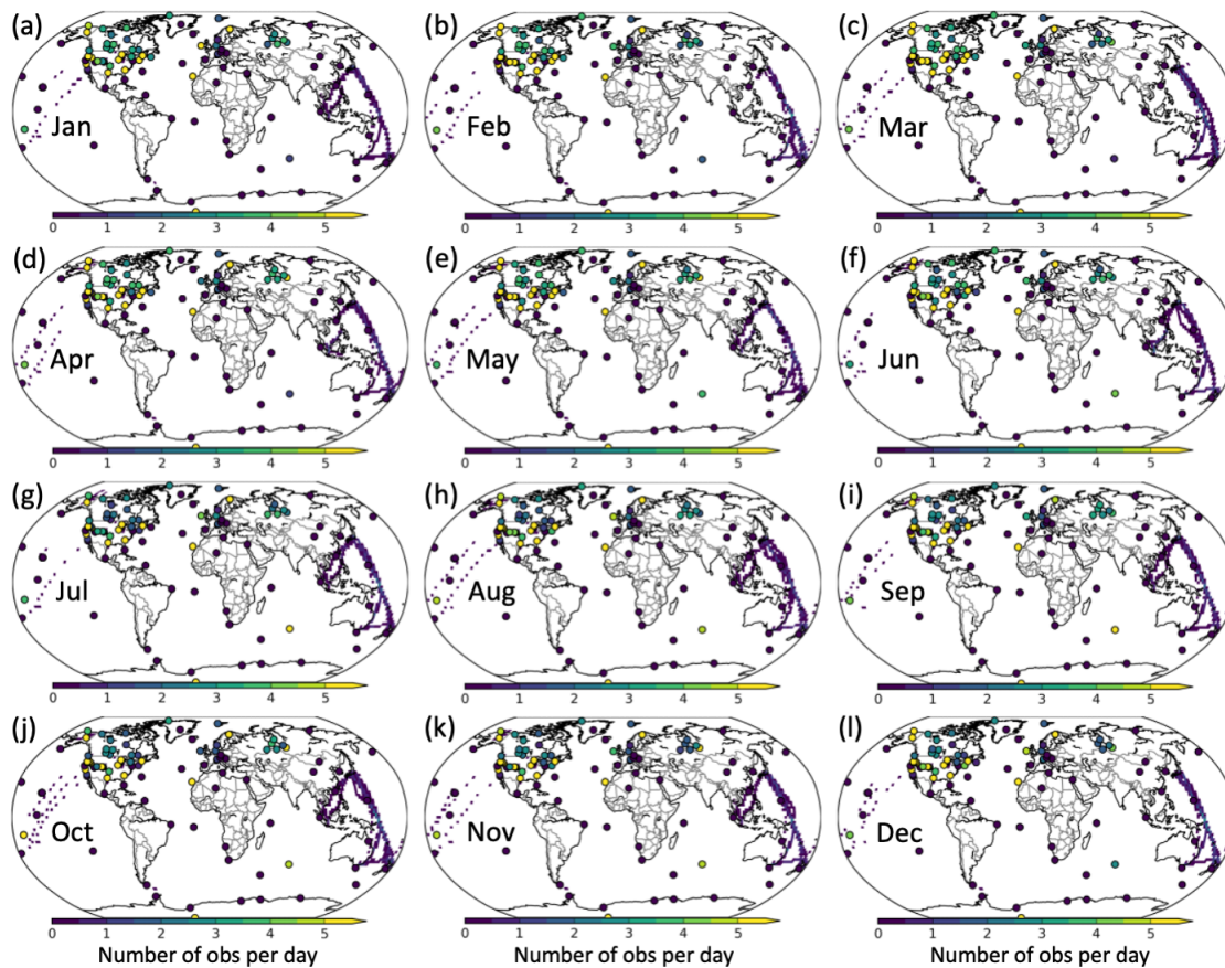
Figure S8. Spatial coverage of monthly in situ and flask measurements averaged over four years (2015, 2016, 2018, and 2019). (a-l) Monthly mean observations per day assimilated in to OCO-2 v10 MIP. Sites are shown by circles while shipboard and aircraft measurements are aggregated to a 1^\circ \times 1^\circ spatial grid.
