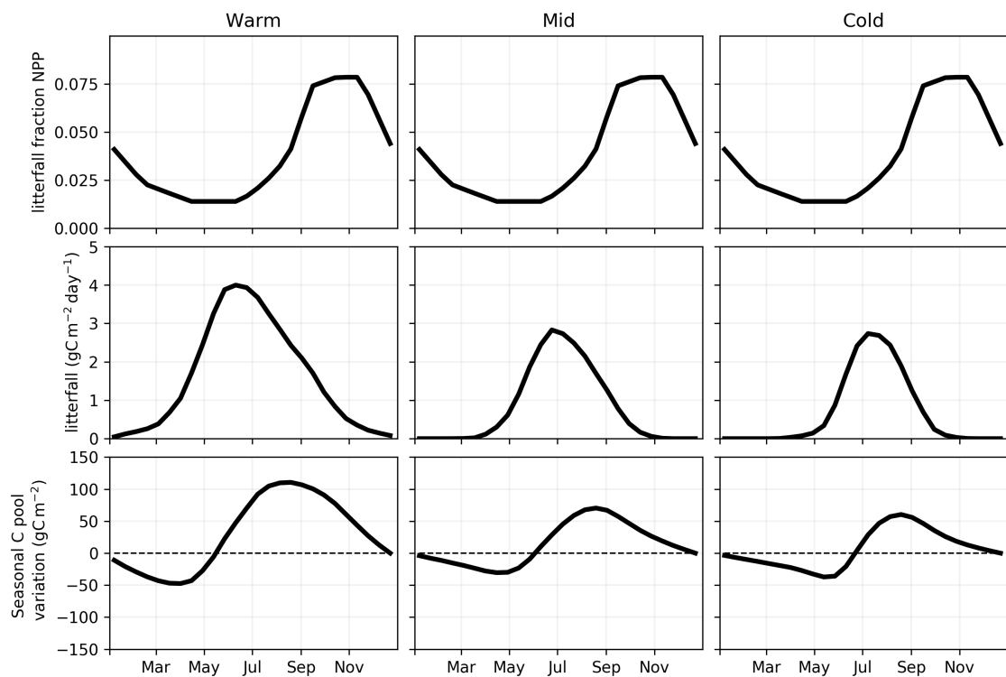
Figure S14. (top) Fraction of NPP that becomes litterfall. (middle row) Carbon flux from litterfall. (bottom) Seasonal variations in the labile carbon pool due to litterfall and R_h .
