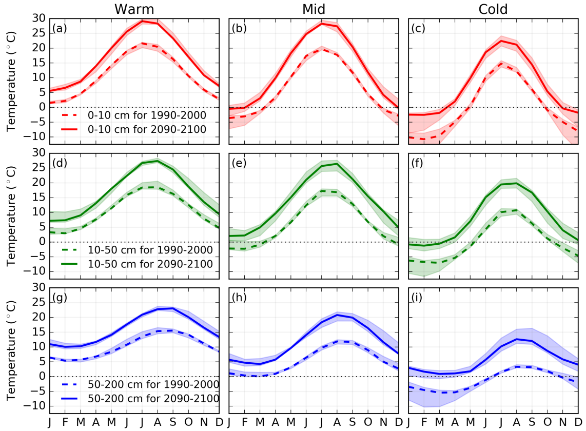
Figure S18. Simulated soil surface temperature for 1990–2000 (dashed) and 2090-2100 (solid) averaged over depths of (a-c) 0–10 cm, (d-f) 10-50 cm and (g-i) 50–200 cm for the three Eurasian regions examined in this study. The lines show the model median and shaded area shows the interquartile spread.
