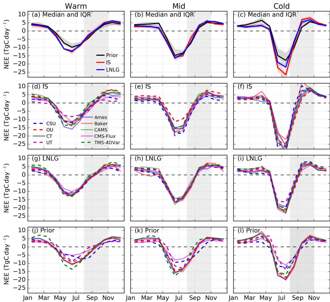
Figure S2. NEE fluxes from individual MIPv9 participants. (a-c) Median and interquartile spread for each experiment. Individual model NEE estimates for the (d-f) IS experiment, (g-i) LNLG experiment, and (j-l) prior fluxes.
