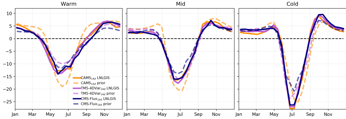
Figure S3. Prior (dashed) and posterior (solid) NEE fluxes at 14 day temporal resolution for CAMS 14d (orange), TM5-4DVar 14d (magenta), and CMS-Flux 14d (navy blue) flux inversions.
