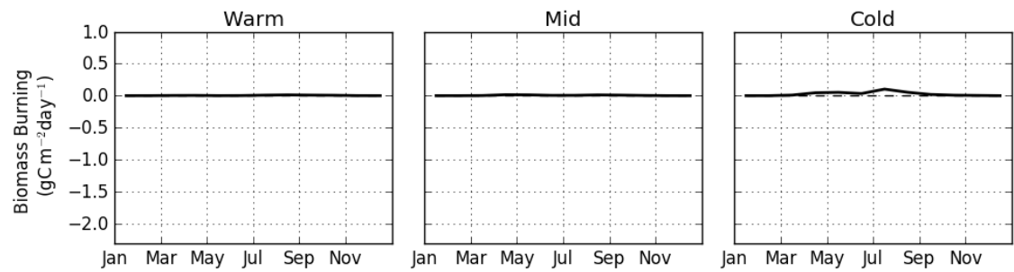
Figure S1. GFED4.1 Biomass burning emissions of CO 2 .
