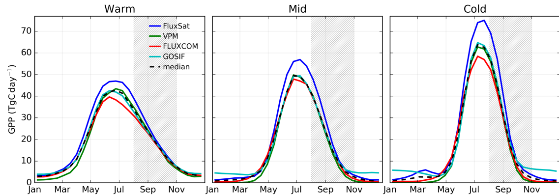
Figure S6. GPP fluxes at 14 day temporal resolution from FluxSat (blue), VPM (green), FLUXCOM (red), and GOSIF (cyan).
