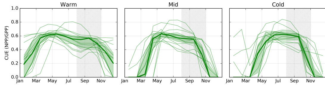
Figure S5. CUE (NPP/GPP) for the TRENDY models. Thin green lines show the CUE for individual models while the thick green line shows the median and shaded regions shows the interquartile spread.
