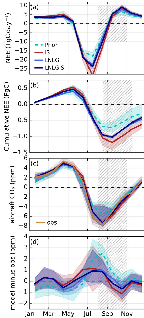
Figure S10. Comparison of flux inversions and aircraft \text{CO}_2 measurements over Alaska. (a) Prior (dashed) and LNLGIS (solid) monthly NEE over the cold region. Shaded areas show the range from the three prior NEE estimates employed in the CMS-Flux 14d inversions. (b) Cumulative NEE \text{CO}_2 flux since the beginning of the year. (c) Mean observed (brown) and simulated atmospheric \text{CO}_2 seasonal cycle for airborne measurements over Alaska. (d) Monthly mean simulated \text{CO}_2 measurements minus the observations over Alaska.
