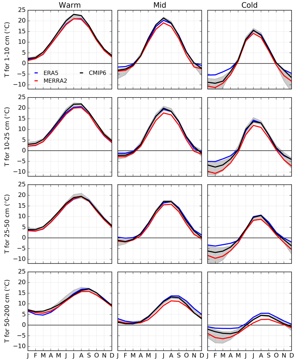
Figure S13. Seasonal cycle of soil temperature for three regions and four different depth intervals (1–10 cm, 10–25 cm, 25–50 cm, 50–200 cm) estimated by MERRA-2 Land, ERA5 Land, and CMIP6 models. MERRA-2 (red) and ERA5 (blue) seasonal cycles are calculated as the mean over 2010–2019. For CMIP6, the mean seasonal cycle over 2010–2019 is calculated for each model, then the model median (solid black) and interquartile range (shaded grey) are plotted across the seven models included in this analysis.
