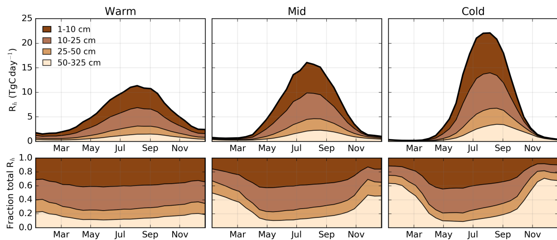
Figure S17. Seasonal cycle of R_h from four soil carbon layers simulated by the soil carbon decomposition model.
