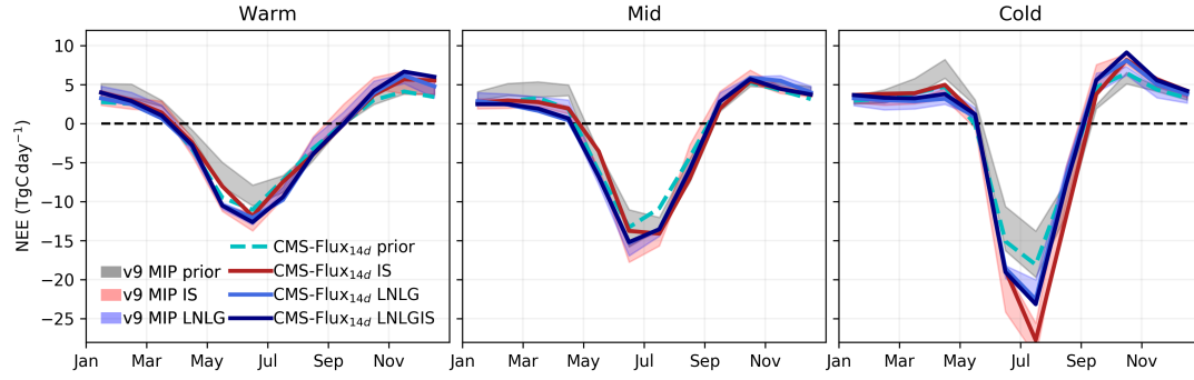
Figure S9. Seasonal cycle of NEE for the OCO-2 MIPv9 and CMS-Flux 14d flux inversions at monthly temporal resolution over the (a) warm, (b) mid, and (c) cold regions. The shaded regions show the interquartile spread for the MIPv9 prior (grey), IS (red) and LNLG (blue) ensembles. The lines show the CMS-Flux 14d prior (dashed cyan), IS (red), LNLG (blue), and LNLGIS (navy).
