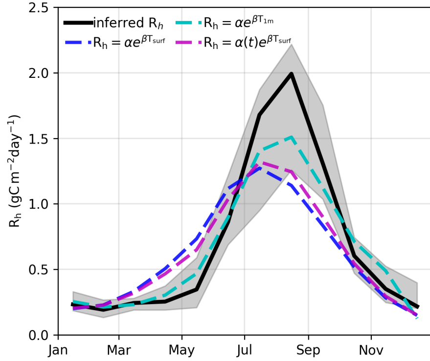
Figure S15. Mean and range in inferred monthly FLUXNET R_h with fits for single-layer R_h models that employ (navy dash) T_{surf} dependence and no seasonal variations in the carbon pool, (cyan dash) T_{1m} dependence and no seasonal variations in the carbon pool and (magenta dash) T_{surf} dependence and seasonal variations in the carbon pool.
