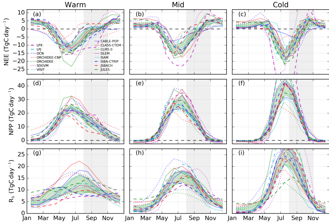
Figure S4. (a-c) NEE, (d-f) NPP, and (g-i) R_h seasonal cycles simulated by each TRENDY v8 model examined in this study. The shaded green area shows the TRENDY model interquartile spread, while individual lines show specific models: (dash magenta) LPX, (dashed cyan) LPJ, (dotted blue) OCN, (dotted red) ORCHIDEE-CNP, (dotted green) ORCHIDEE, (dotted magenta) SDGVM, (dotted cyan) VISIT, (solid blue) CABLE-POP, (solid red) CLASS-CTEM, (solid green) CLM5.0, (solid magenta) DLEM, (solid cyan) ISAM, (dashed blue) ISBA-CTrip, (dashed red) JSBACH, and (dashed green) JULES.
